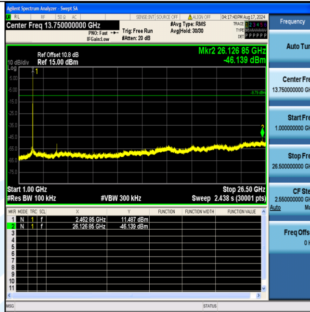
11B-Ant2-2462-1000~26500-PASS
