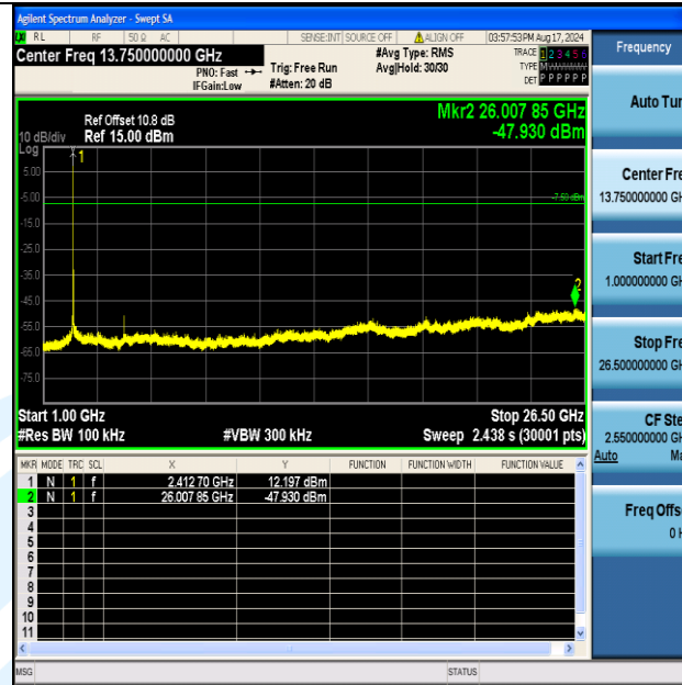
11B-Ant2-2412-1000~26500-PASS
