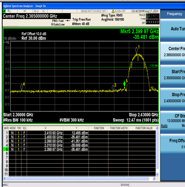
11B-Ant2-2412-PASS
