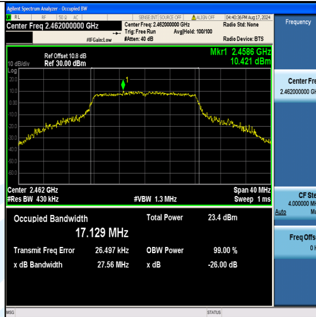
11G-Ant2-2462
