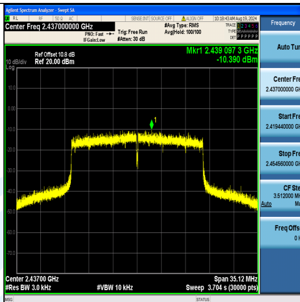
11AX20MIMO-Ant2-2437-PASS
