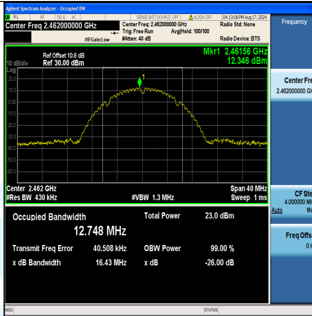
11B-Ant2-2462
