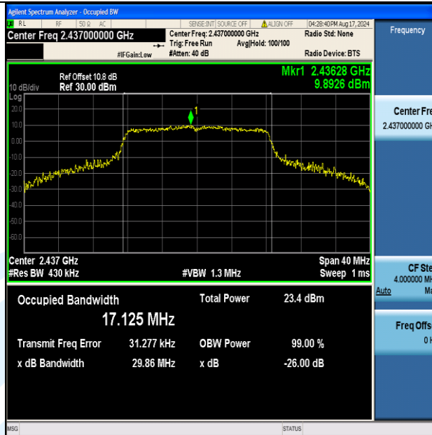
11G-Ant2-2437
