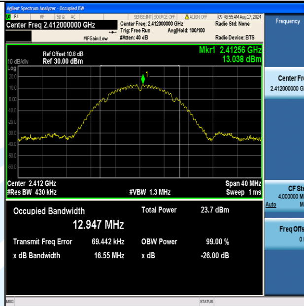
11B-Ant2-2412
