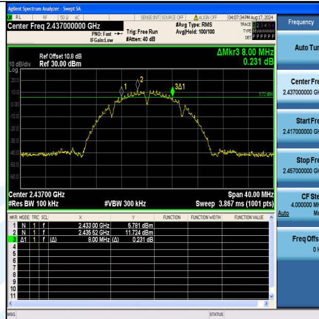
11B-Ant2-2437-PASS
