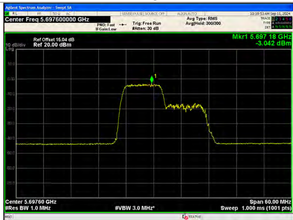
PSD NVNT ax40 106@53 5710MHz Ant2
