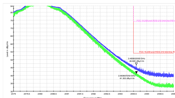
Figure 8.3-7: Upper band edge emission within restricted bands at 2.4835 GHz
