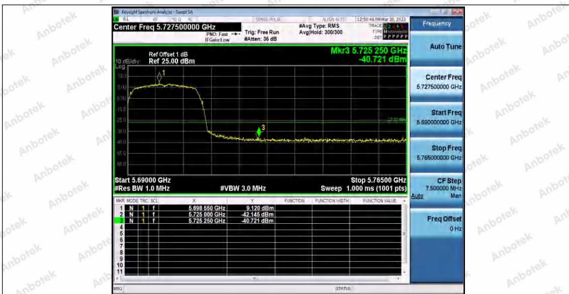
11N20SISO_Ant2_High_5700
