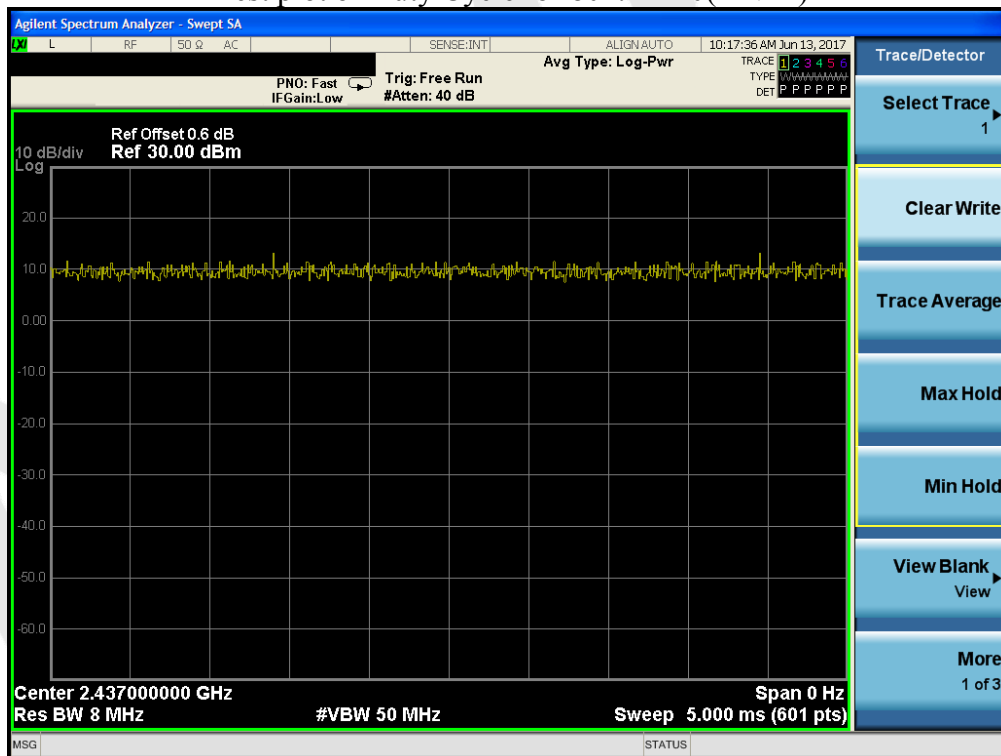
Test plot of Duty Cycle for 802.11n40(ANT1)
