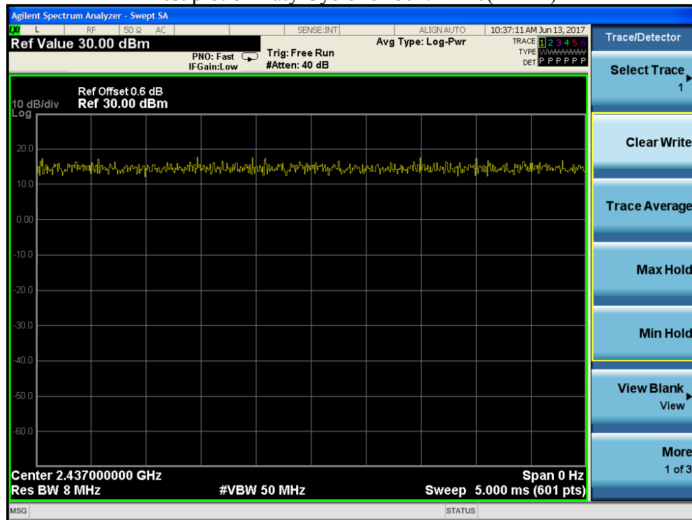
Test plot of Duty Cycle for 802.11n20(ANT2)
