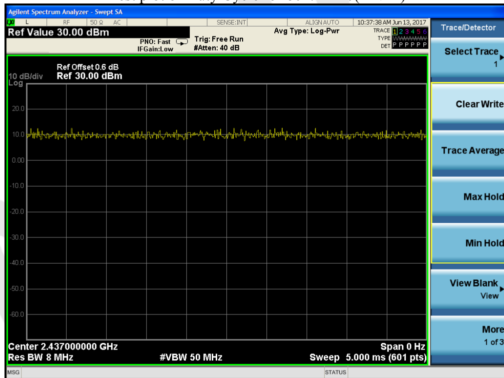
Test plot of Duty Cycle for 802.11n40(ANT2)
