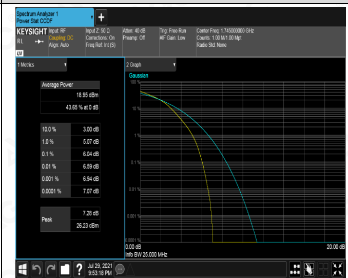
HCH_16QAM_100RB#0
