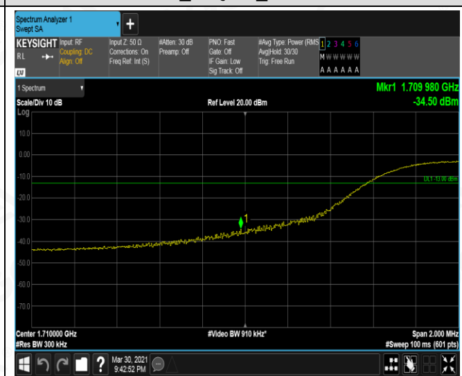
HCH_16QAM_75RB#0
