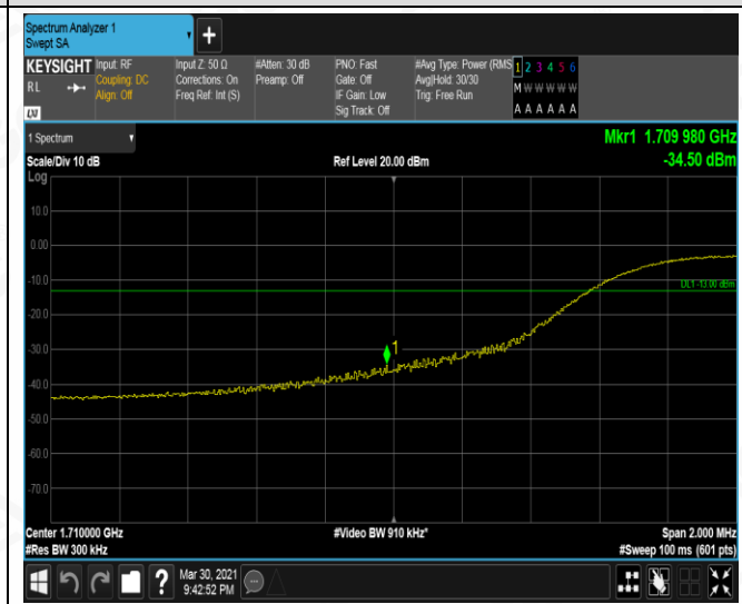
LCH_16QAM_75RB#0
