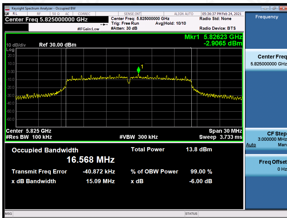
Test_Graph_802.11a_ANT1_5825_6Mbps_DTSBW
