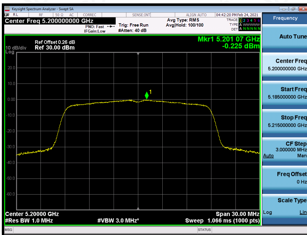
Test_Graph_802.11n20_ANT1_5200_MCS0_PSD
