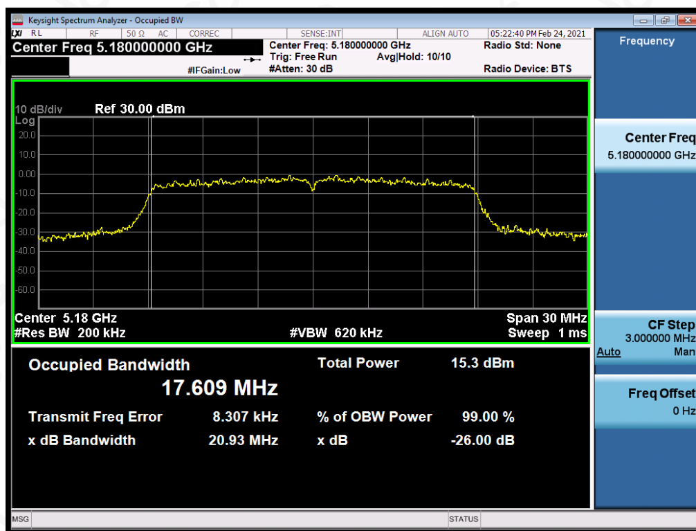
Test_Graph_802.11ac20_ANT1_5180_MCS0_OBW
