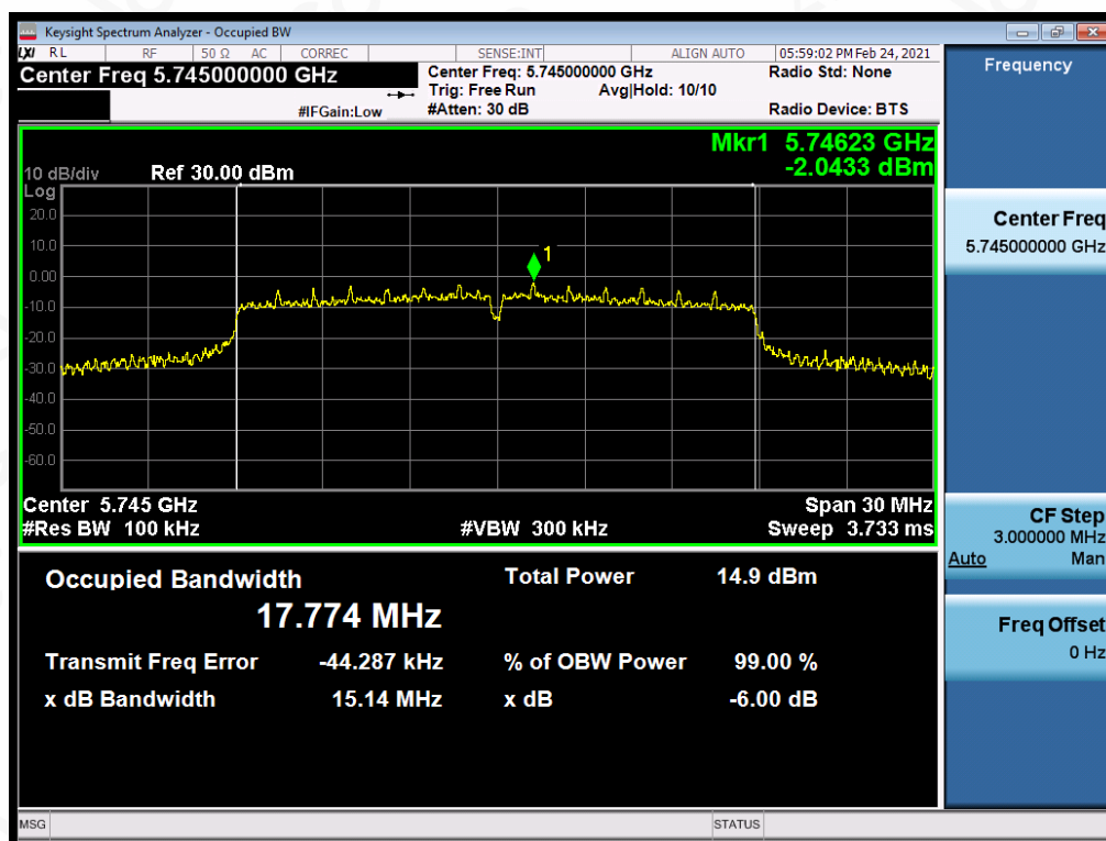
Test_Graph_802.11ac20_ANT1_5745_MCS0_DTSBW
