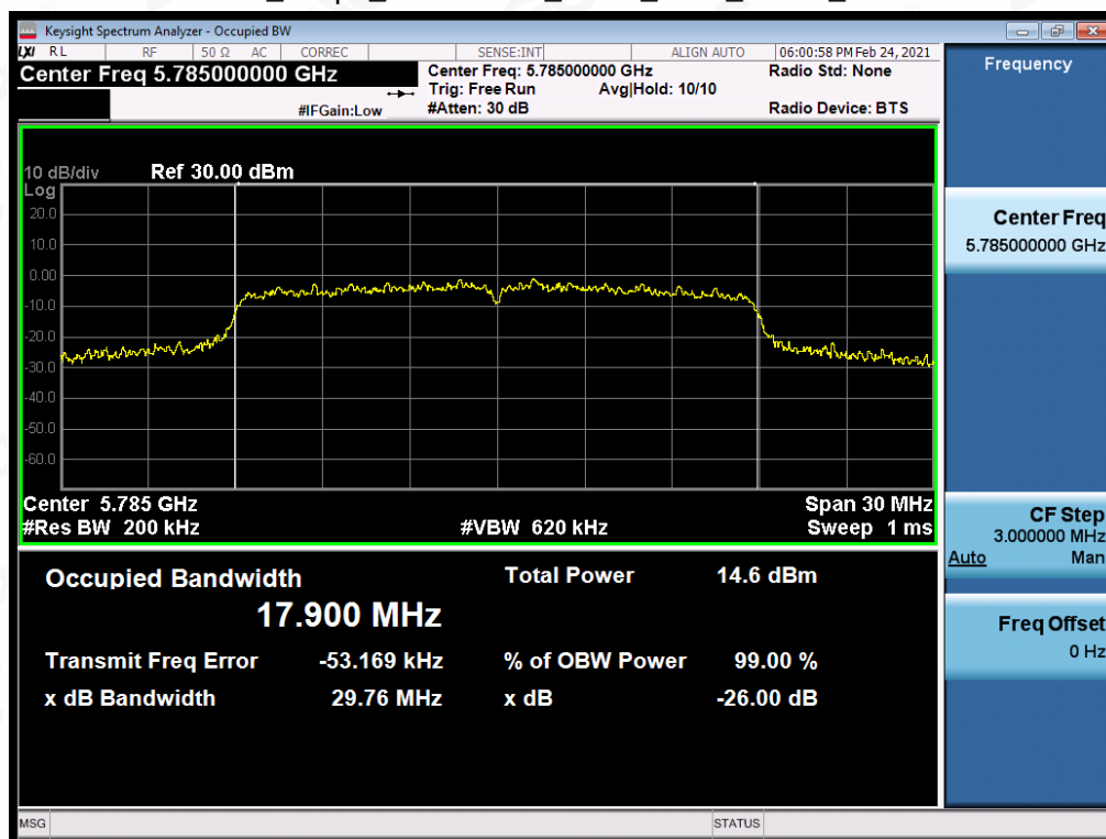
Test_Graph_802.11ac20_ANT1_5785_MCS0_OBW
