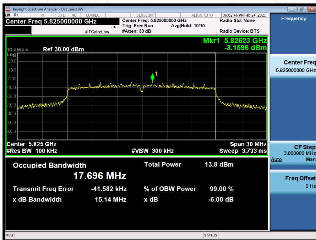
Test_Graph_802.11ac20_ANT1_5825_MCS9_DTSBW
