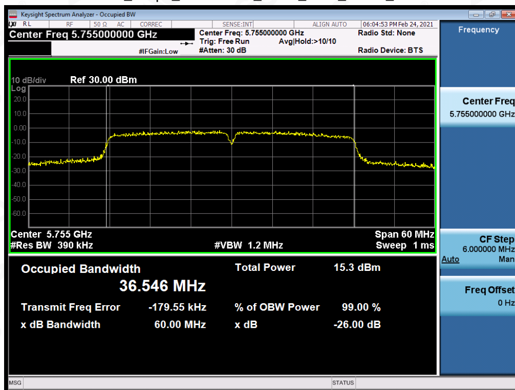
Test_Graph_802.11ac40_ANT1_5755_MCS9_OBW
