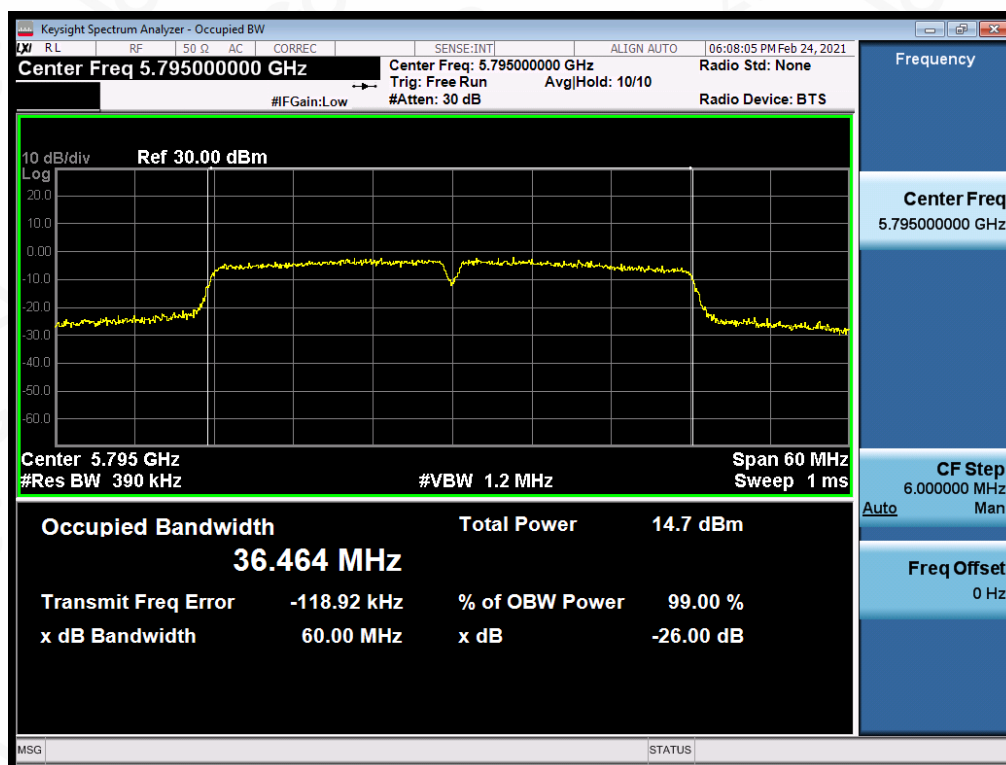
Test_Graph_802.11ac40_ANT1_5795_MCS9_OBW
