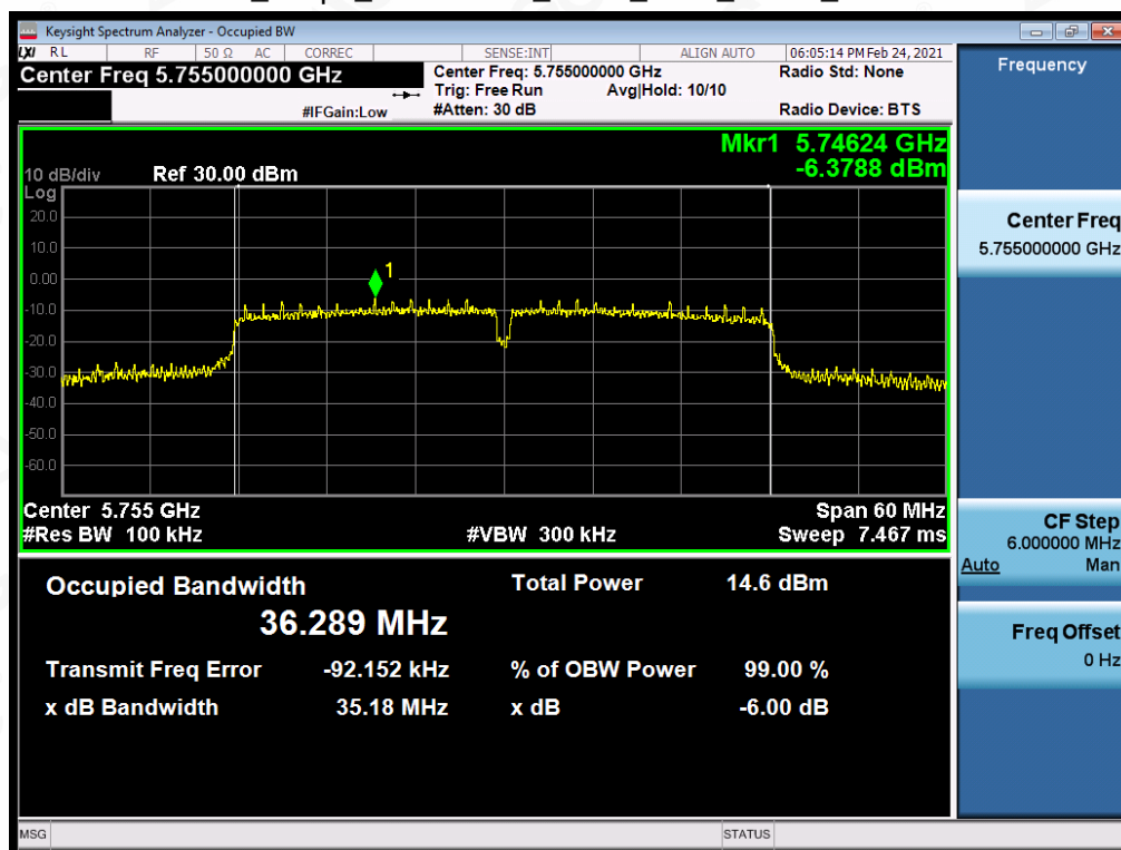
Test_Graph_802.11ac40_ANT1_5755_MCS9_DTSBW
