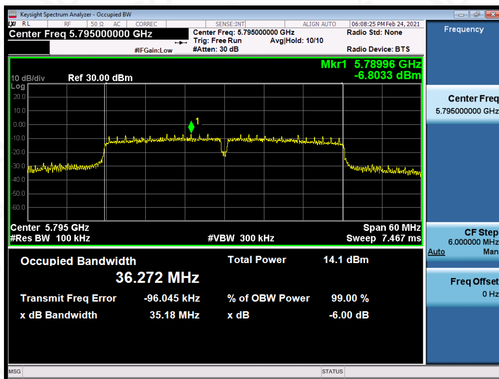
Test_Graph_802.11ac40_ANT1_5795_MCS9_DTSBW
