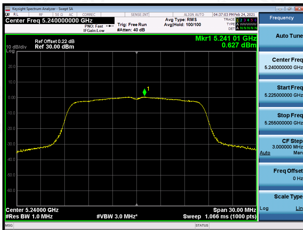
Test_Graph_802.11a_ANT1_5240_6Mbps_PSD
