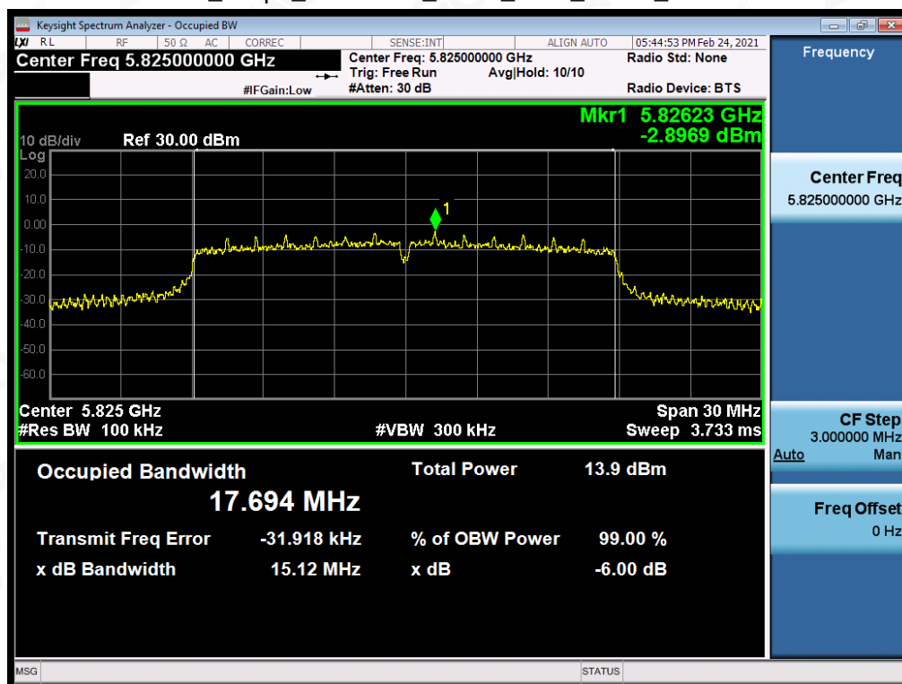
Test_Graph_802.11n20_ANT1_5825_MCS0_DTSBW
