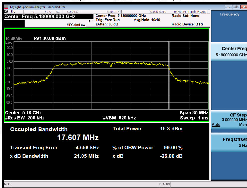
Test_Graph_802.11n20_ANT1_5180_MCS0_OBW
