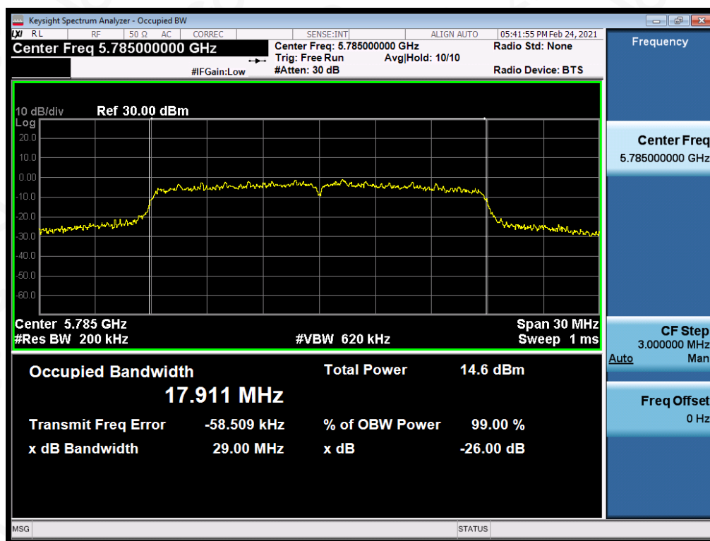
Test_Graph_802.11n20_ANT1_5785_MCS0_OBW
