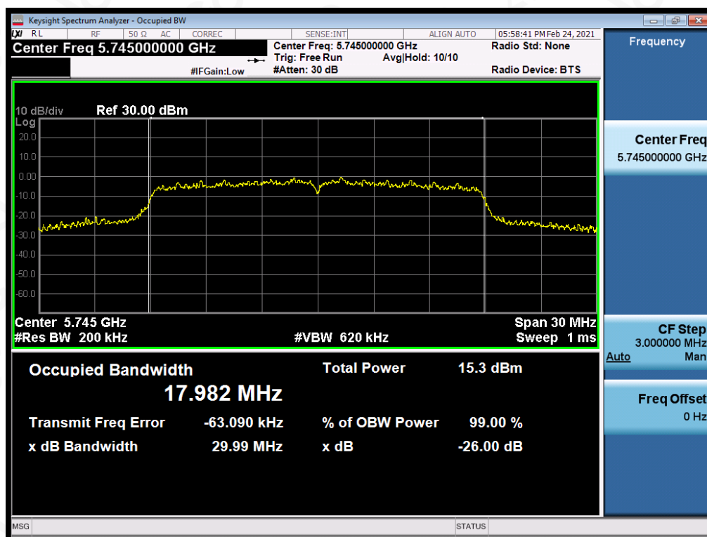
Test_Graph_802.11ac20_ANT1_5745_MCS0_OBW
