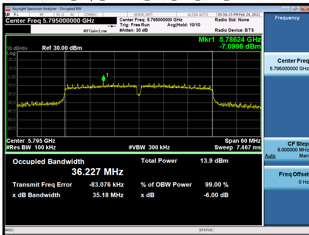
Test_Graph_802.11n40_ANT1_5795_MCS0_DTSBW
