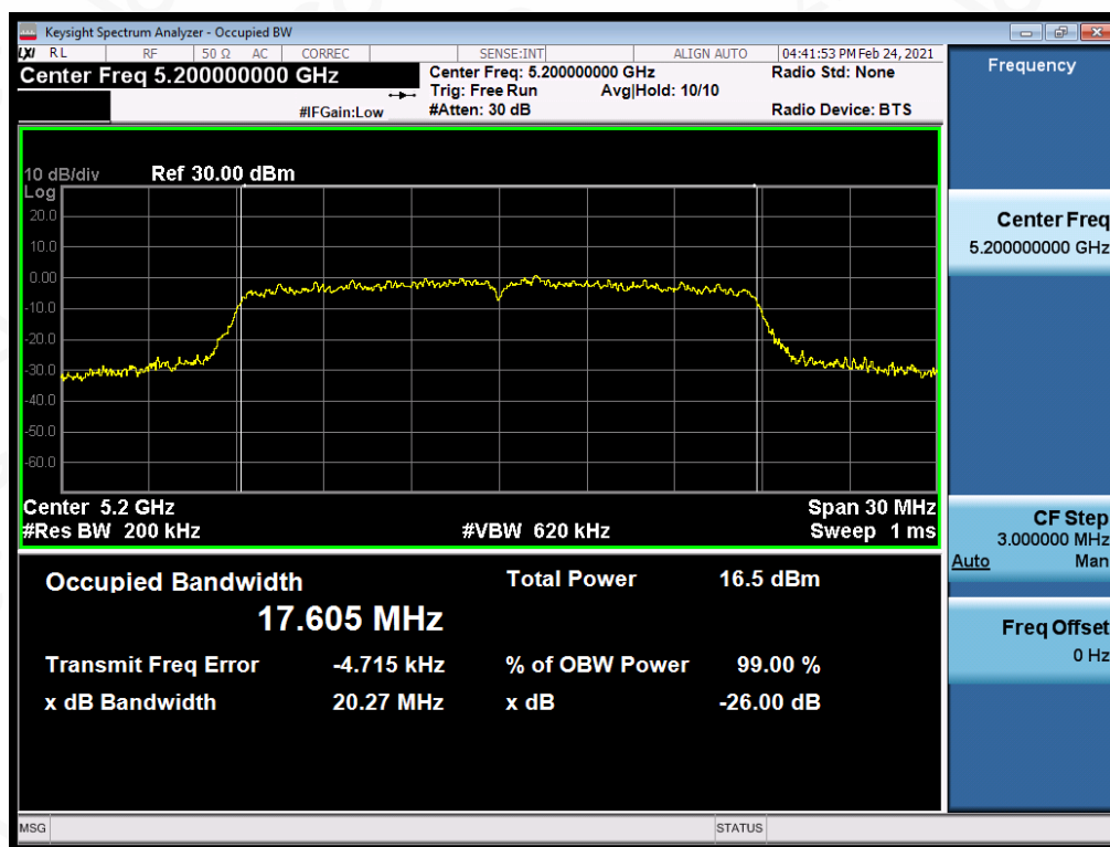
Test_Graph_802.11n20_ANT1_5200_MCS0_OBW
