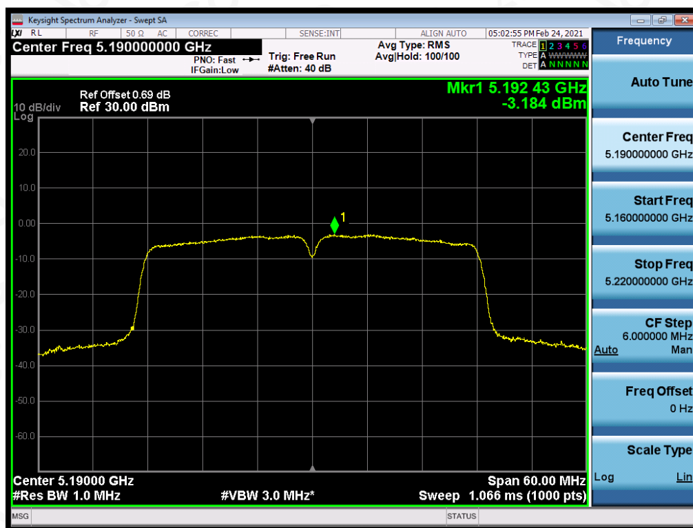
Test_Graph_802.11n40_ANT1_5190_MCS0_PSD
