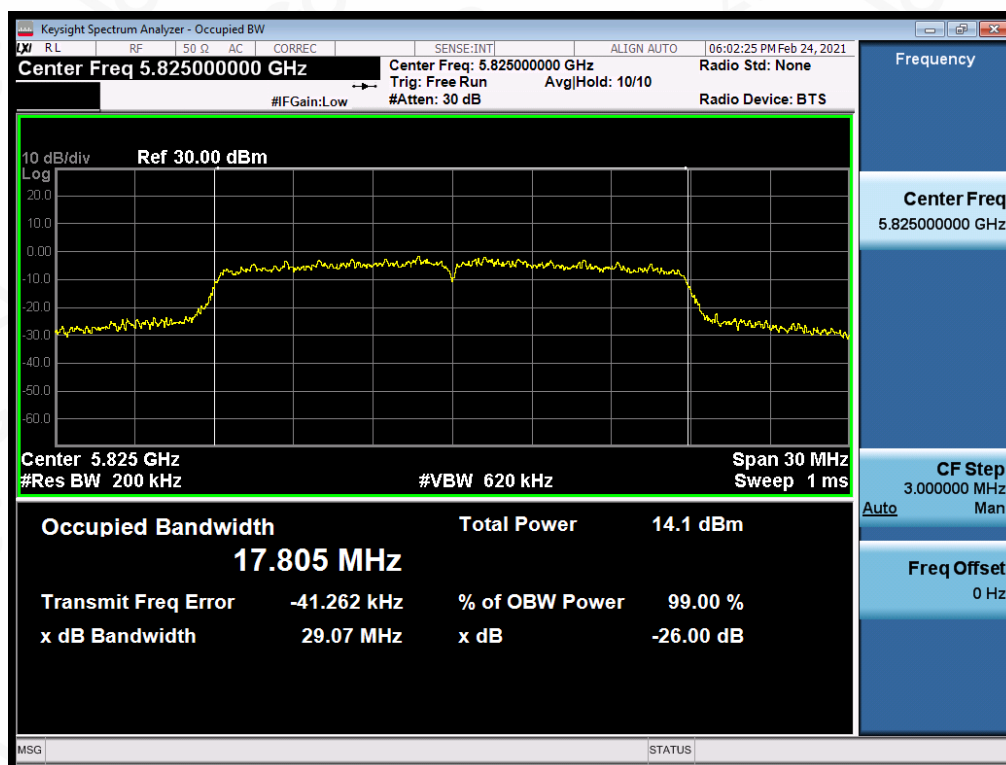
Test_Graph_802.11ac20_ANT1_5825_MCS9_OBW
