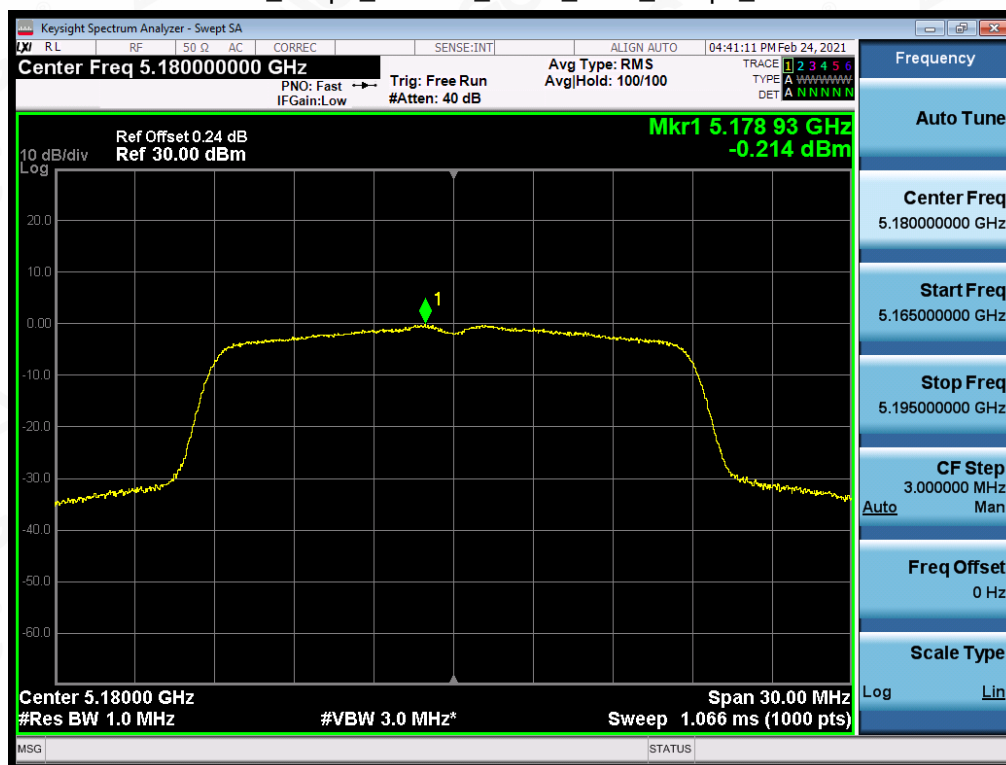
Test_Graph_802.11n20_ANT1_5180_MCS0_PSD
