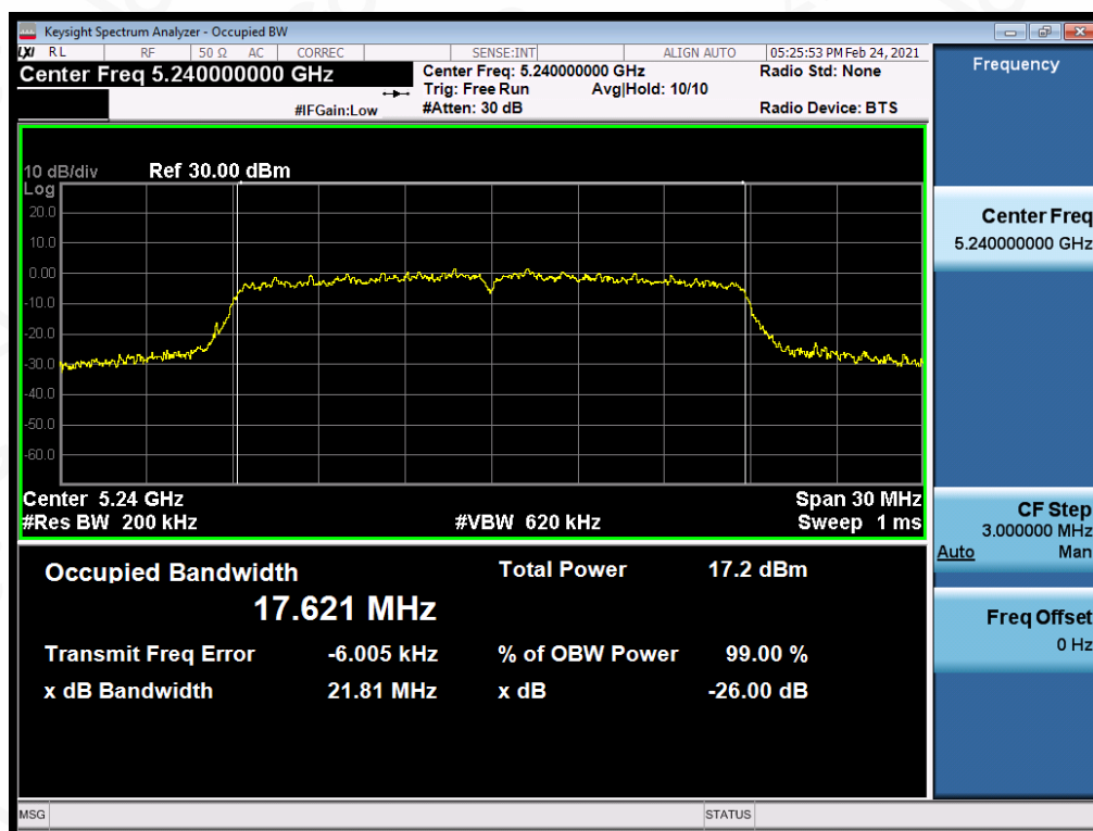
Test_Graph_802.11ac20_ANT1_5240_MCS9_OBW
