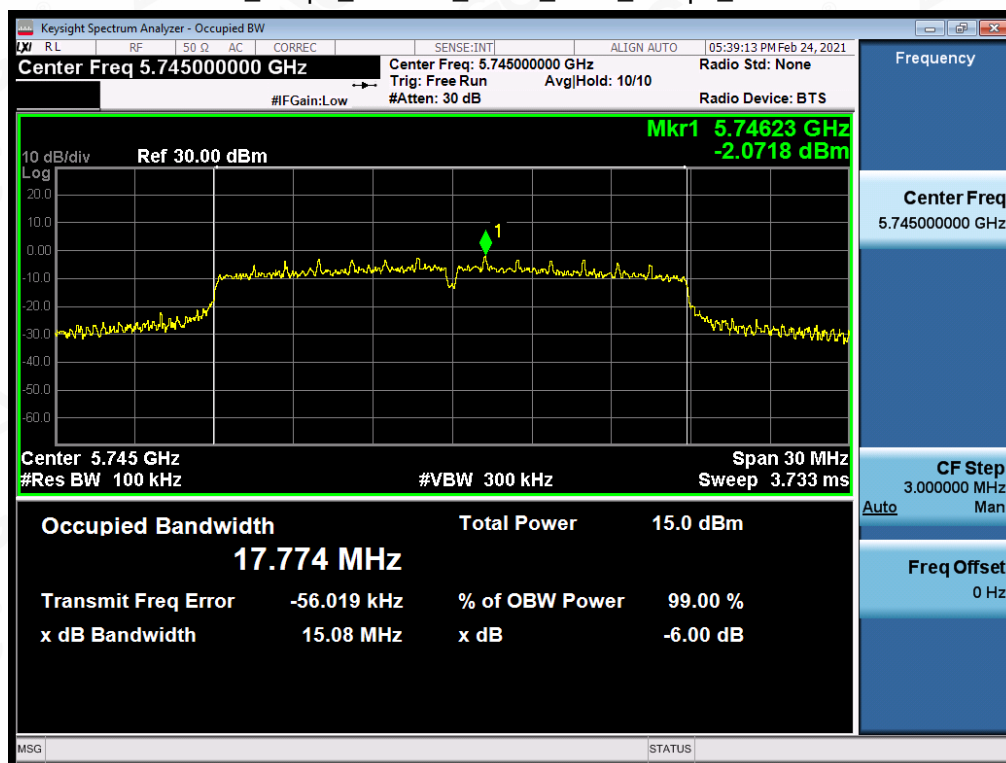
Test_Graph_802.11n20_ANT1_5745_MCS0_DTSBW
