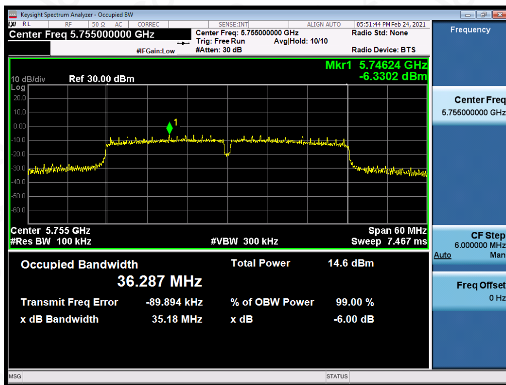
Test_Graph_802.11n40_ANT1_5755_MCS0_DTSBW
