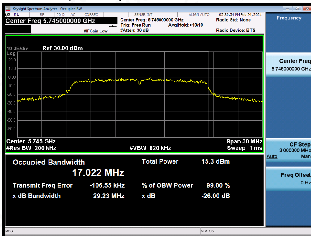
Test_Graph_802.11a_ANT1_5745_6Mbps_OBW
