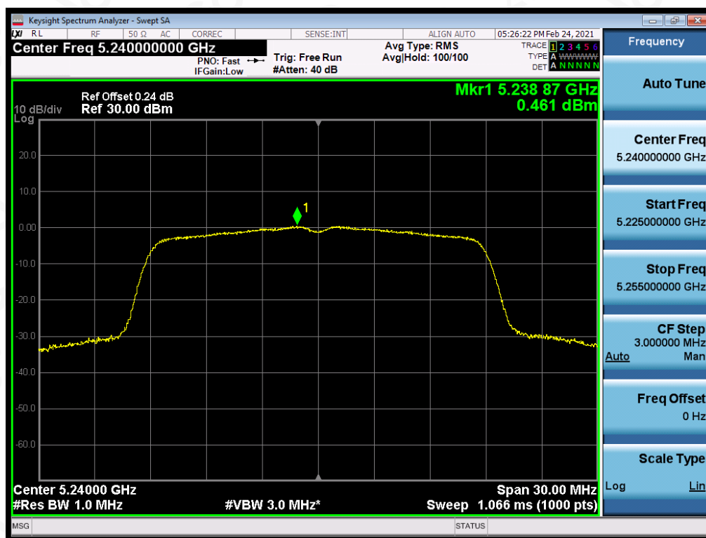
Test_Graph_802.11ac20_ANT1_5240_MCS9_PSD
