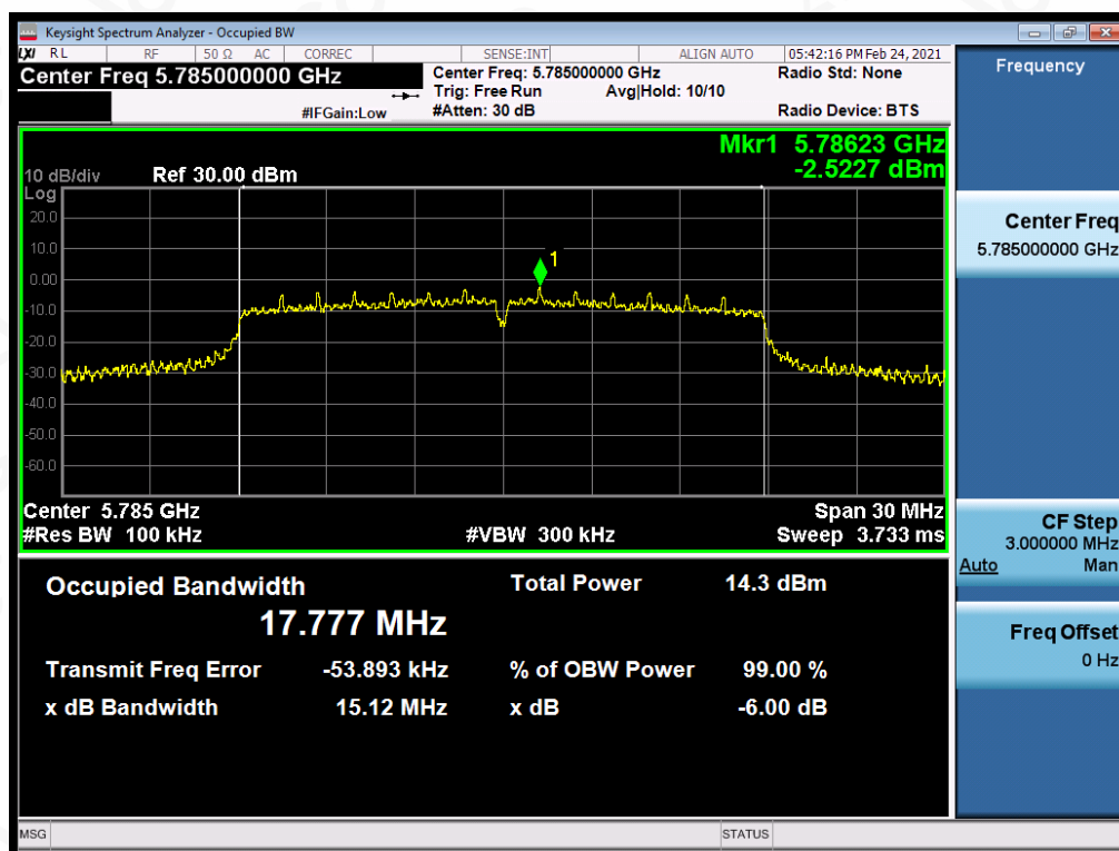
Test_Graph_802.11n20_ANT1_5785_MCS0_DTSBW
