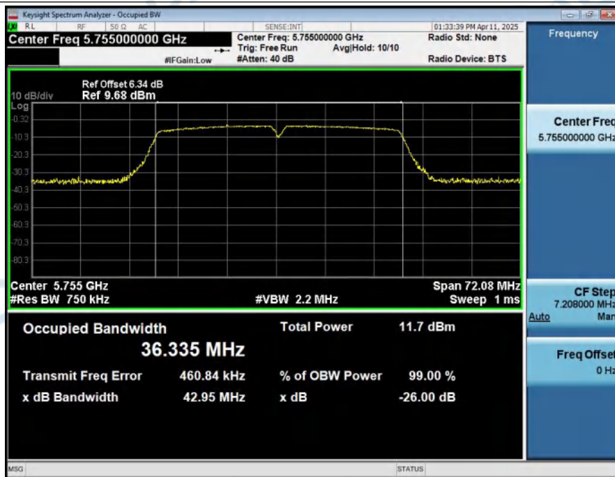
-26BW_NVNT_ANT1_802_11ac(VHT40)_5755
