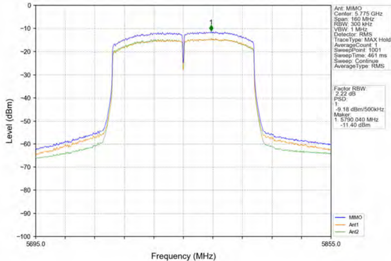
802.11ac(VHT80)_MCH_5775MHz_MIMO_NTNV
