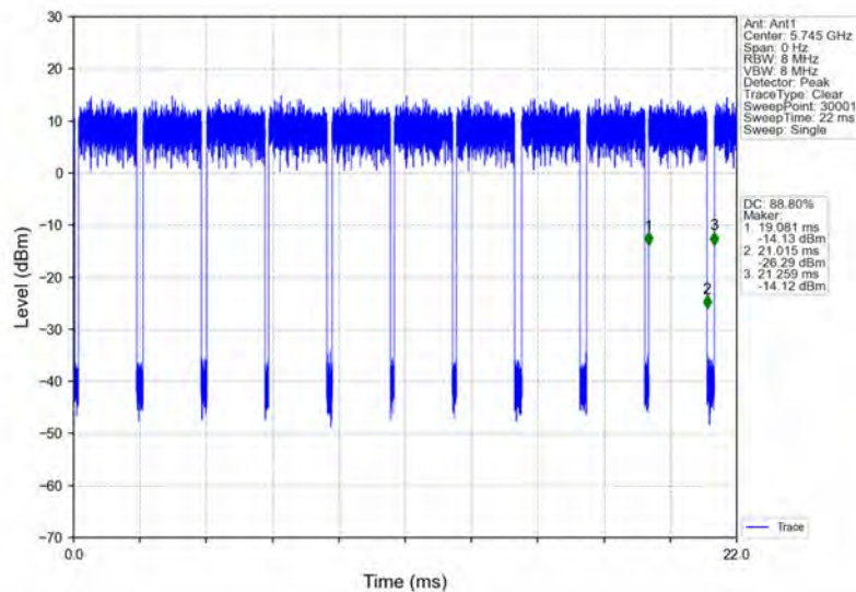
802.11ac(VHT20)_LCH_5745MHz_Ant1_NTNV
