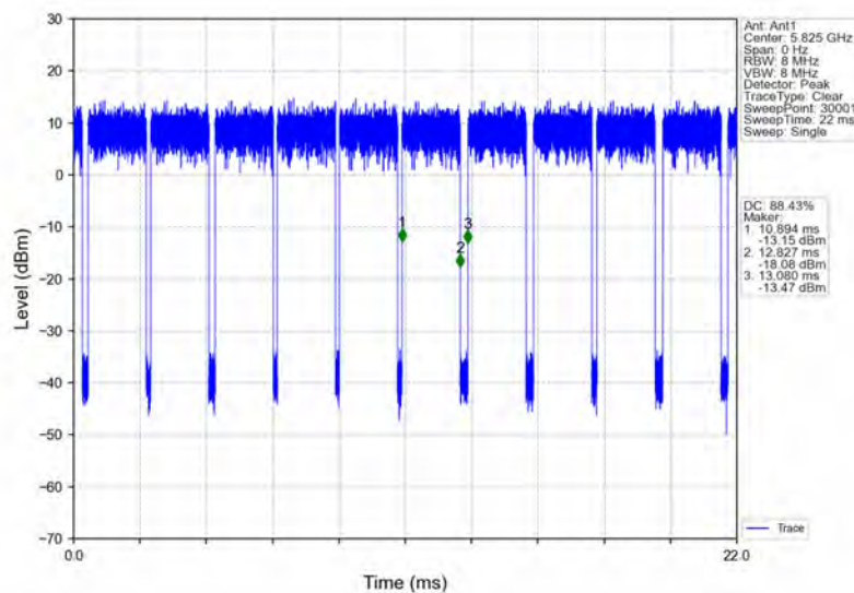
802.11ac(VHT20)_HCH_5825MHz_Ant1_NTNV
