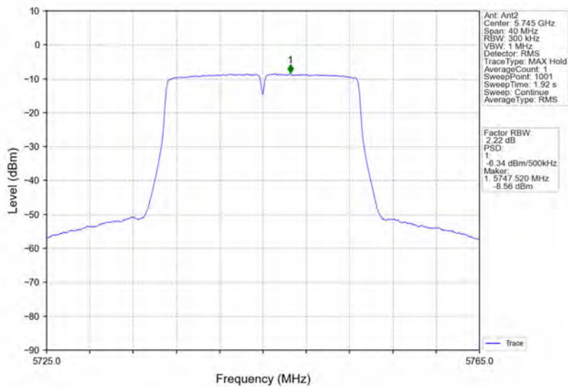
802.11n(HT20)_LCH_5745MHz_Ant2_NTNV
