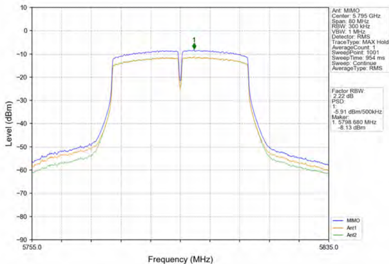
802.11ac(VHT40)_HCH_5795MHz_MIMO_NTNV
