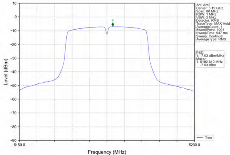
802.11n(HT40)_LCH_5190MHz_MIMO_NTNV
