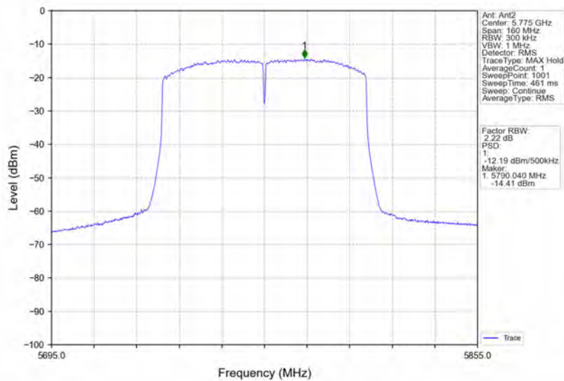
802.11ac(VHT80)_MCH_5775MHz_Ant2_NTNV
