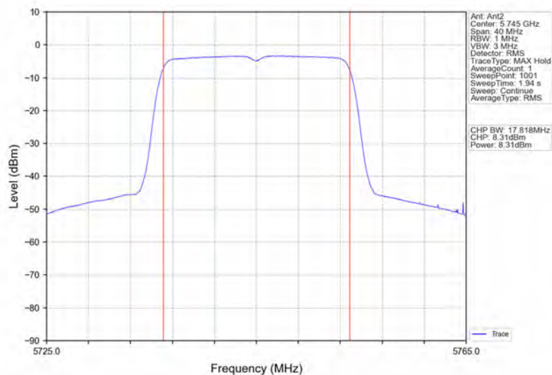
802.11ac(VHT20)_LCH_5745MHz_Ant2_NTNV
