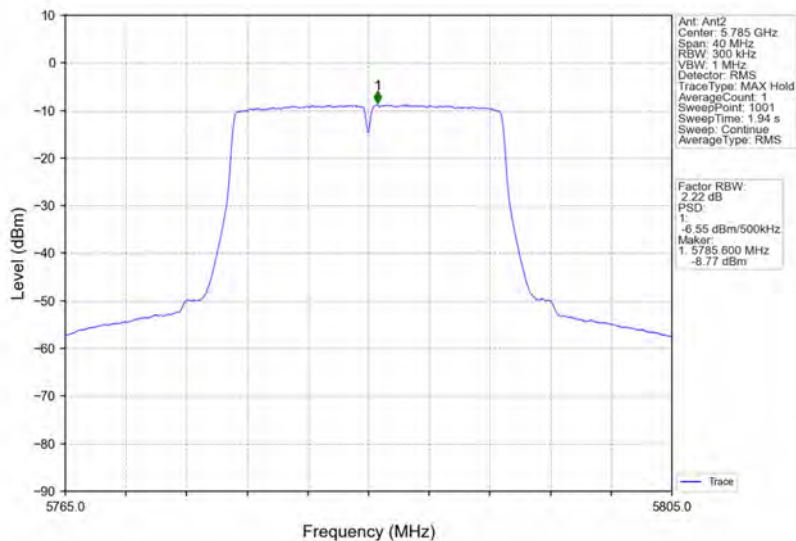
802.11ac(VHT20)_MCH_5785MHz_Ant2_NTNV
