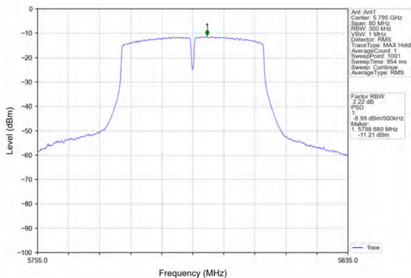
802.11ac(VHT40)_HCH_5795MHz_Ant1_NTNV
