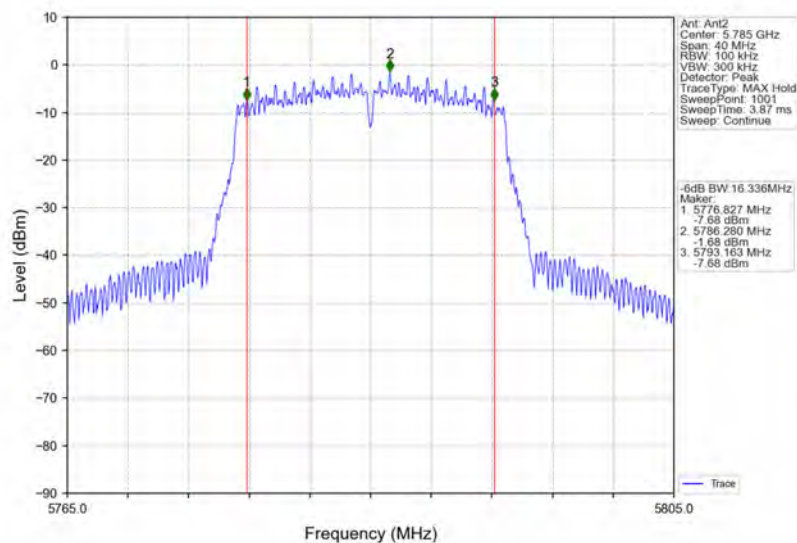
802.11n(HT20)_MCH_5785MHz_Ant2_NTNV
