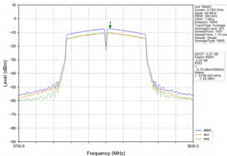
802.11ac(VHT40)_HCH_5795MHz_MIMO_NTNV
