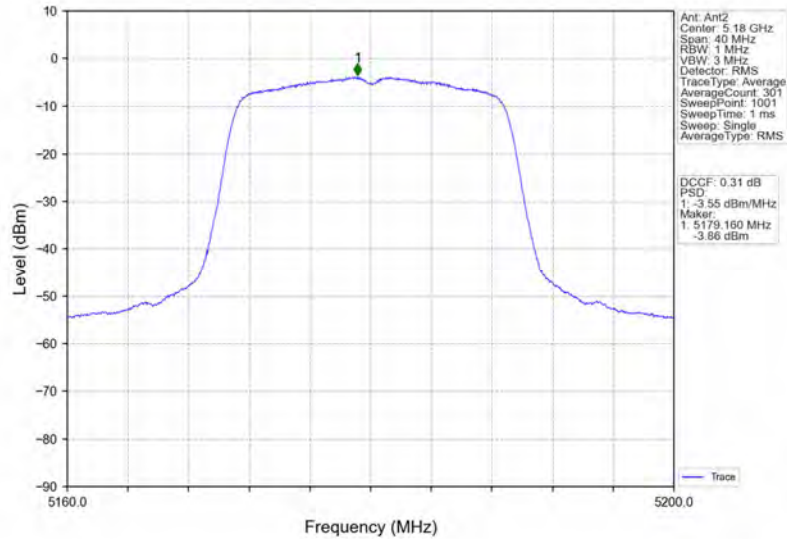
802.11ac(VHT20)_LCH_5180MHz_MIMO_NTNV
