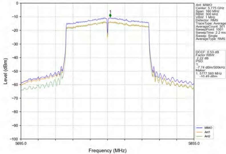
802.11ac(VHT80)_MCH_5775MHz_MIMO_NTNV
