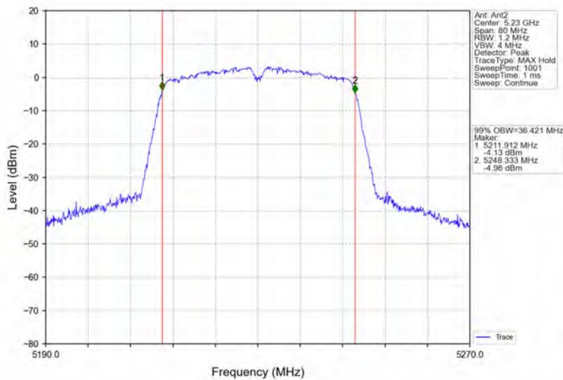
802.11ac(VHT40)_HCH_5230MHz_Ant2_NTNV
