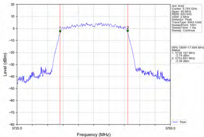
802.11ac(VHT20)_LCH_5745MHz_Ant2_NTNV
