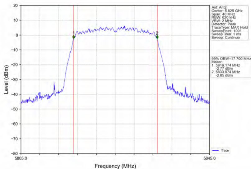
802.11ac(VHT20)_HCH_5825MHz_Ant2_NTNV
