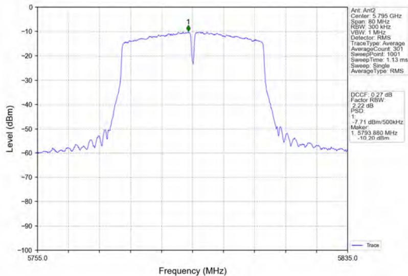
802.11ac(VHT40)_HCH_5795MHz_MIMO_NTNV
