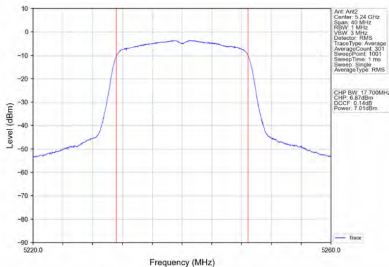
802.11n(HT20)_HCH_5240MHz_Ant2_NTNV
