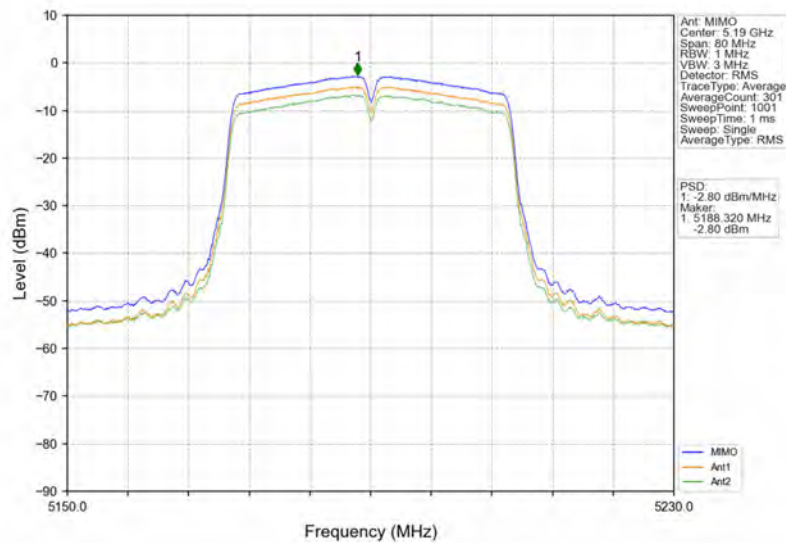
802.11n(HT40)_LCH_5190MHz_MIMO_NTNV
