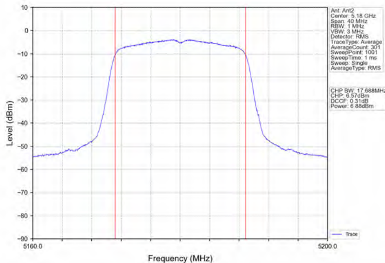
802.11ac(VHT20)_LCH_5180MHz_Ant2_NTNV
