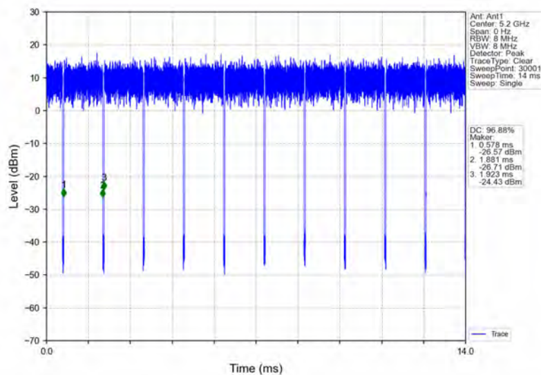
802.11n(HT20)_MCH_5200MHz_Ant1_NTNV
