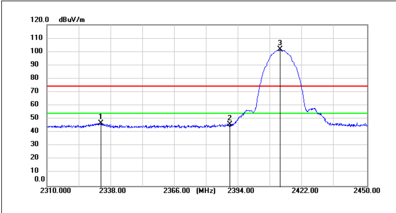
11b_TX_CH_01_Vertical_Peak
