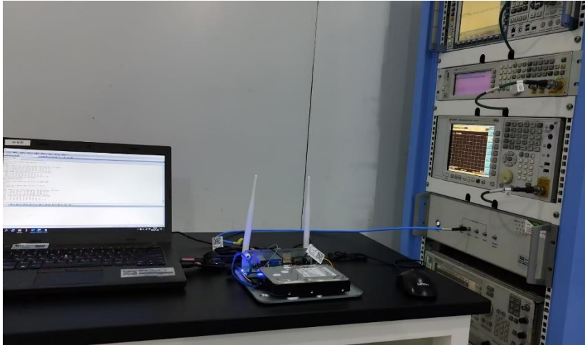
RF conducted setup
