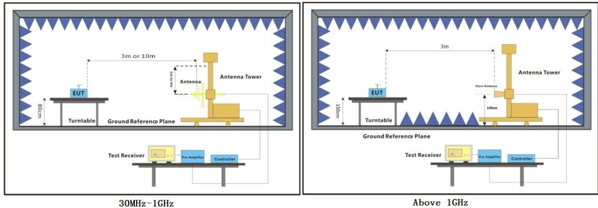
30MHz-1GHz
