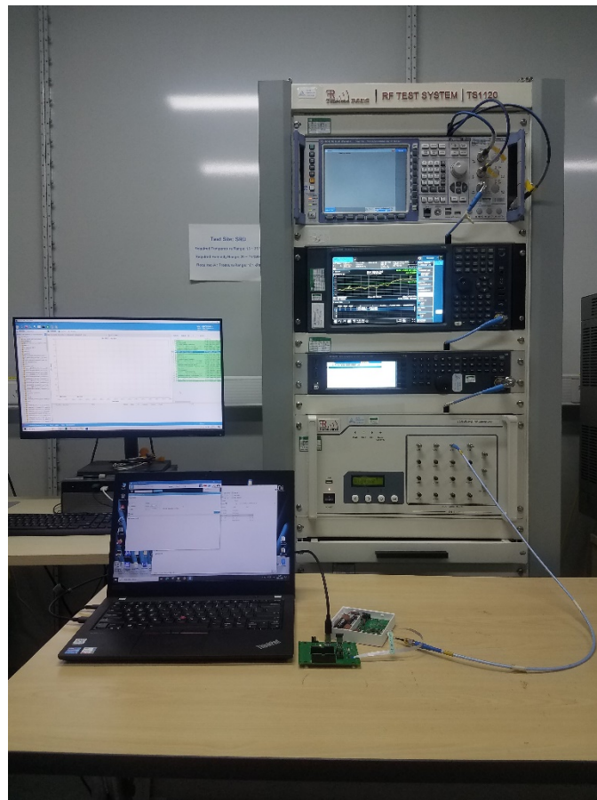
Photograph 3: Set-up photo for Conducted signal test
