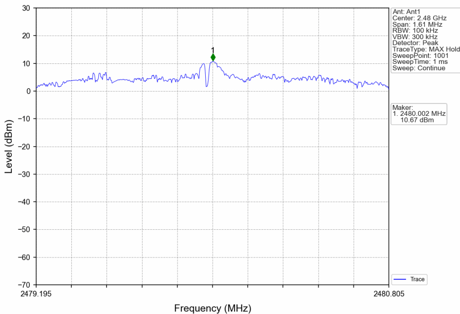
Thread_HCH_2480MHz_Ant1_NTNV
