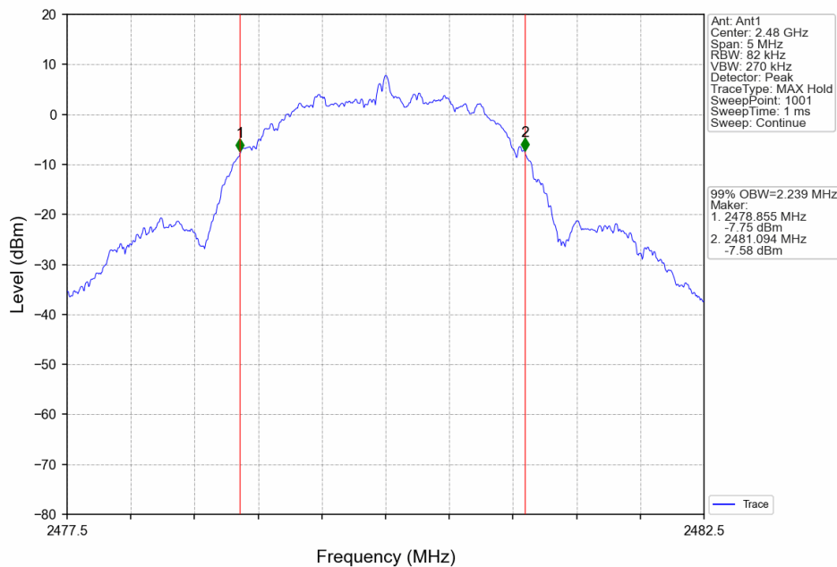
Thread_HCH_2480MHz_Ant1_NTNV
