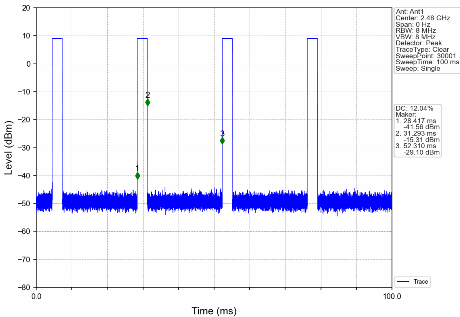
Thread_HCH_2480MHz_Ant1_NTNV
