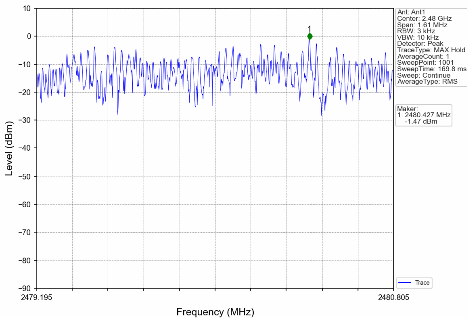
Thread_HCH_2480MHz_Ant1_NTNV
