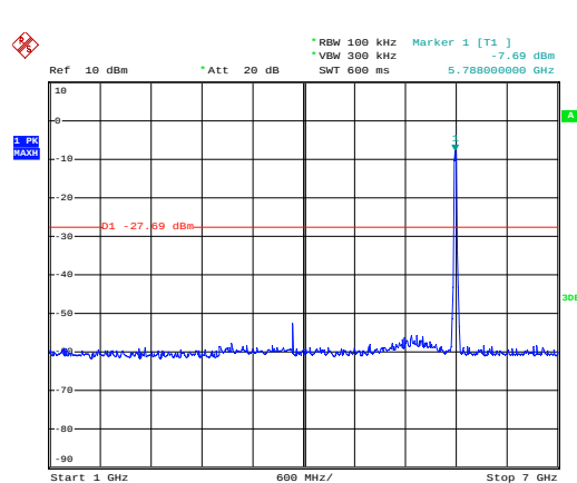
802.11n40 on channel 159
