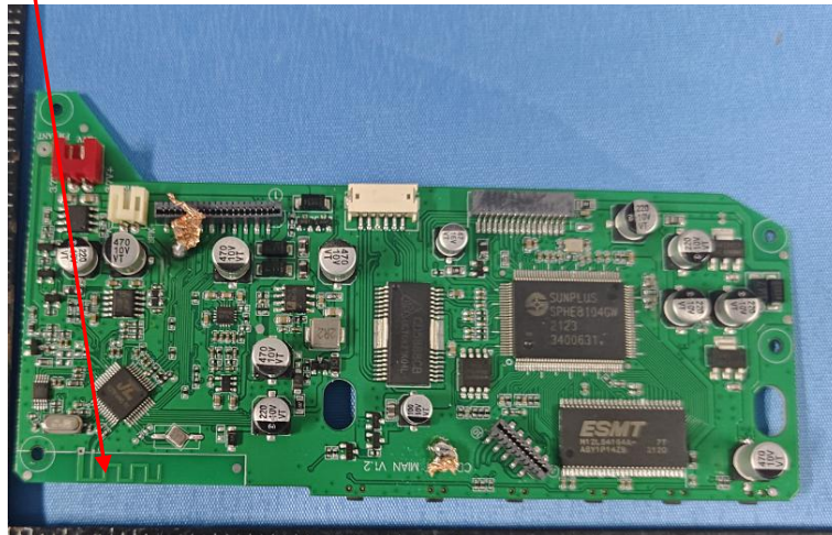
PCB Antenna
