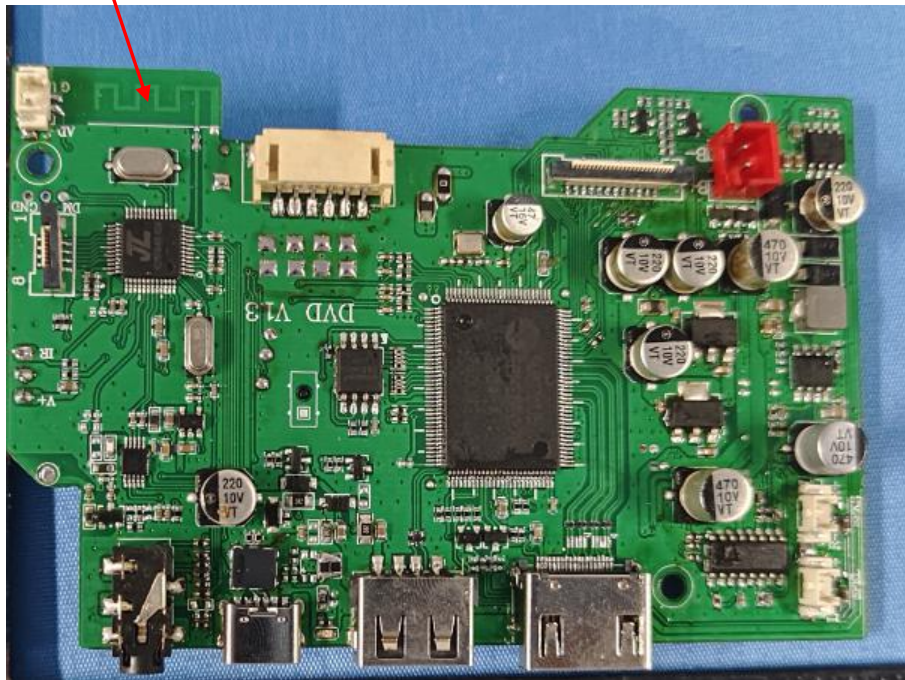
PCB Antenna
