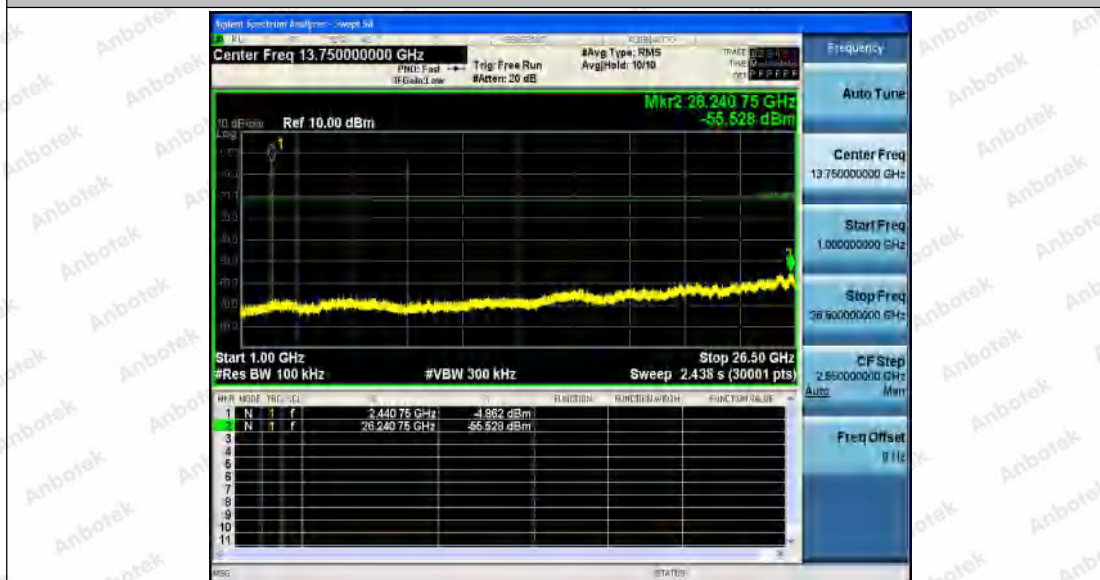
2DH5_Ant1_2441_1000~26500
