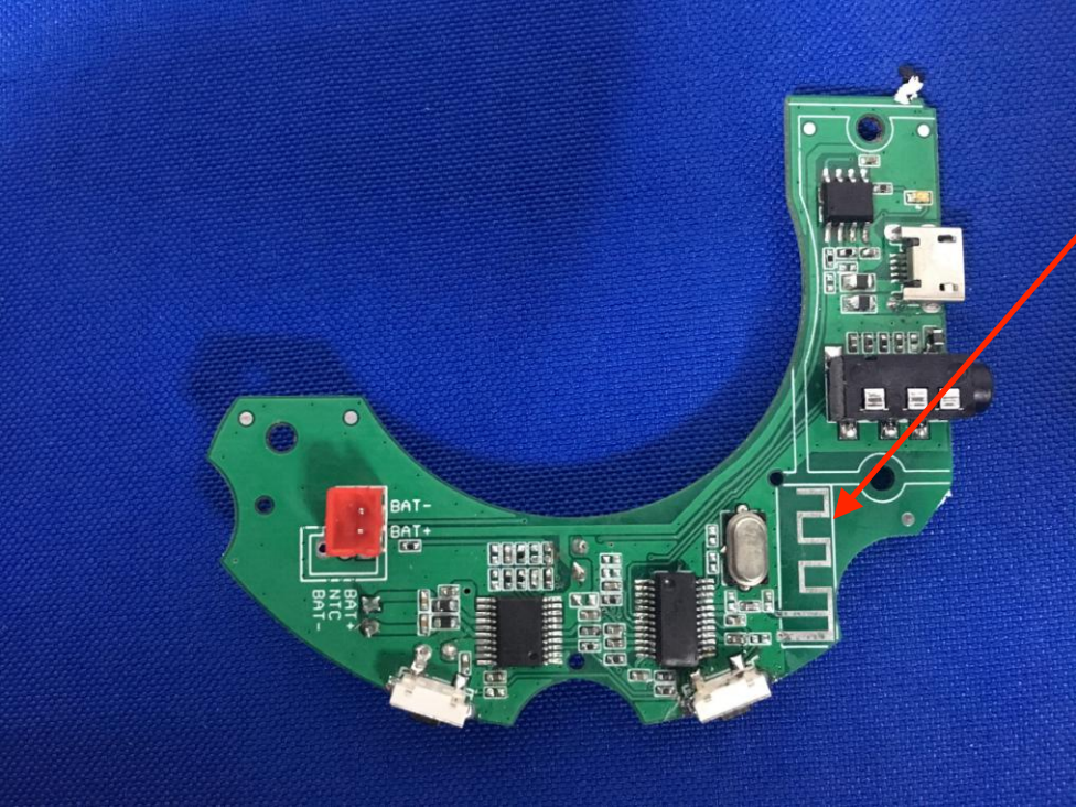
BT Antenna
