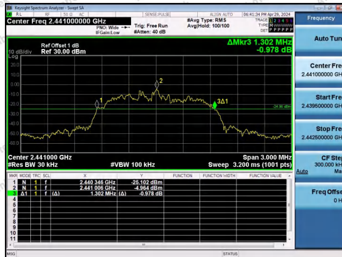
3DH5-Ant1-2441
