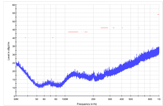
NEX419806 Mid channel RE PK+, MAXH FCC 15.209 and RSS-Gen Restricted bands average limits
