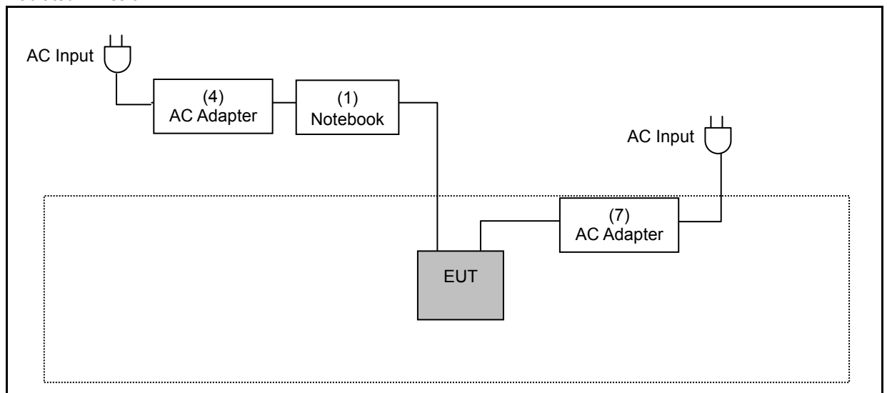
Radiated Emission
