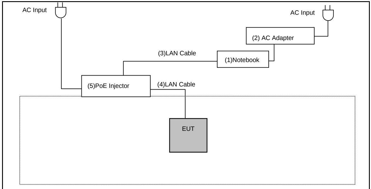
Conducted Emission
