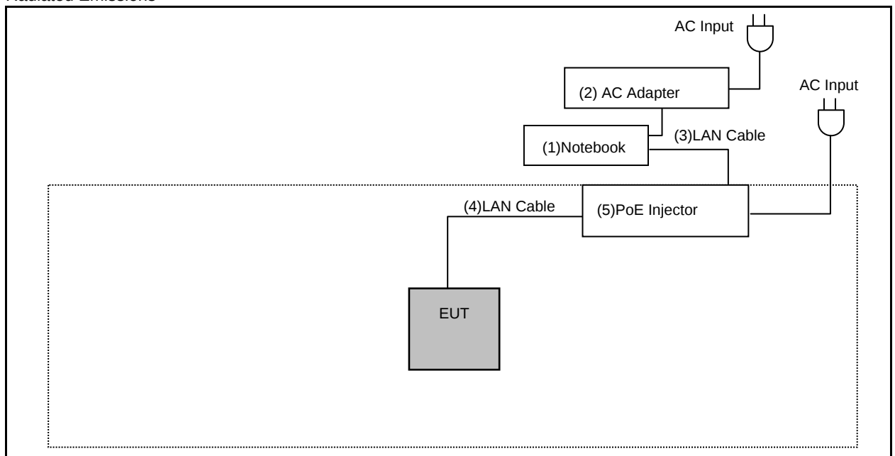
Radiated Emissions
