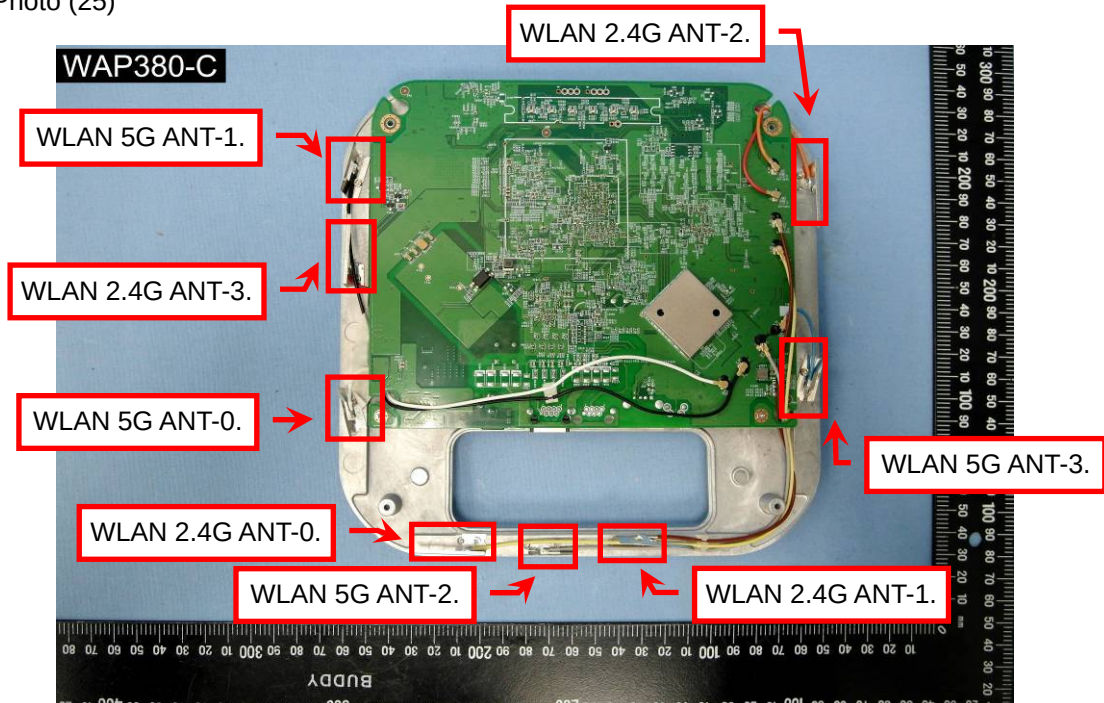
EUT Photo (25)
