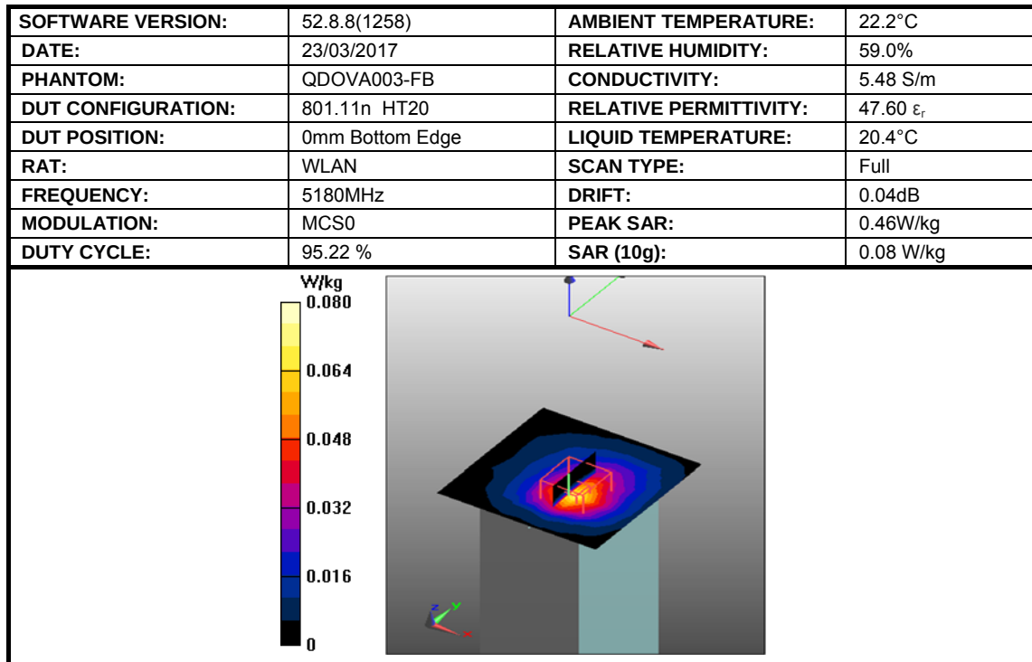
Figure 27: SAR Head Testing Results for the BCF Technology Ltd Duo Scan:Go at 5180 MHz
