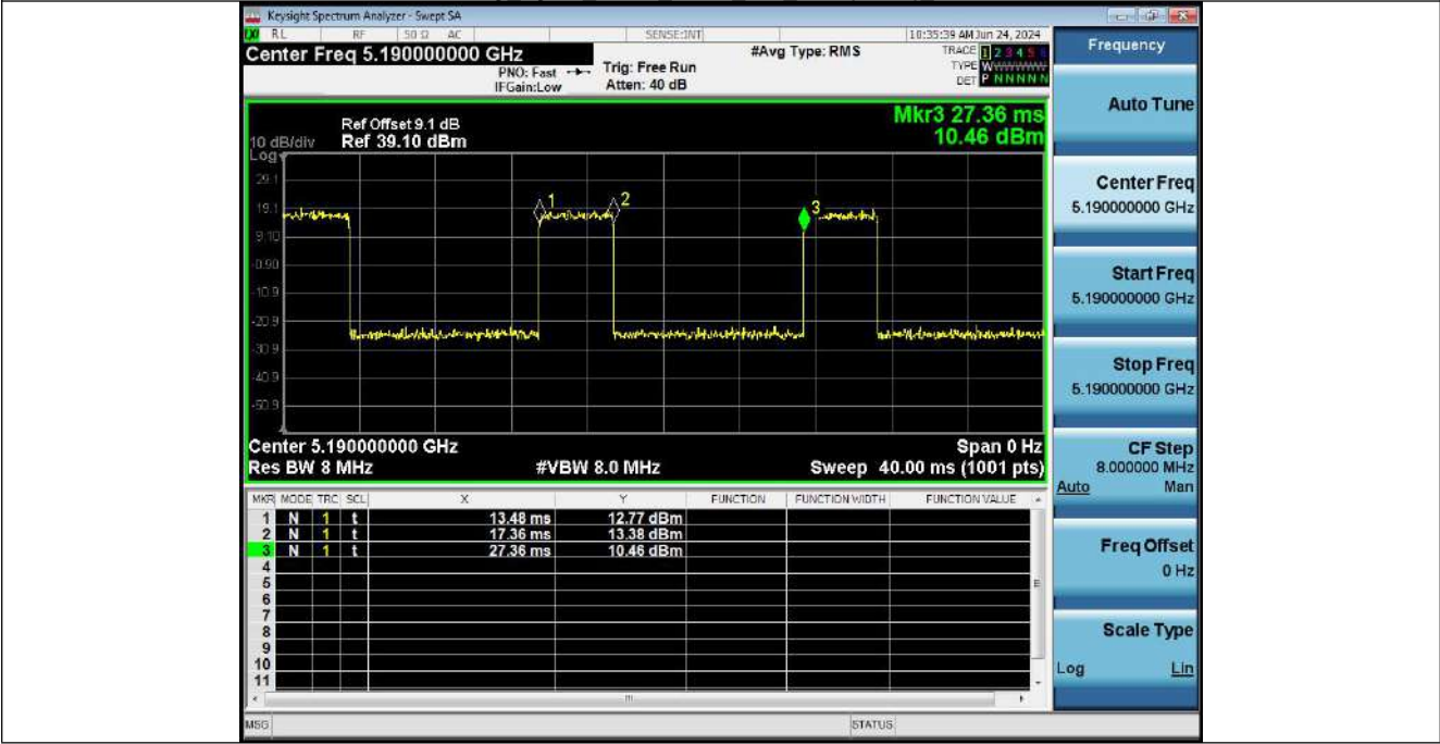
Duty Cycle_NVNT_ANT1_802_11ax(HE40)_5190
