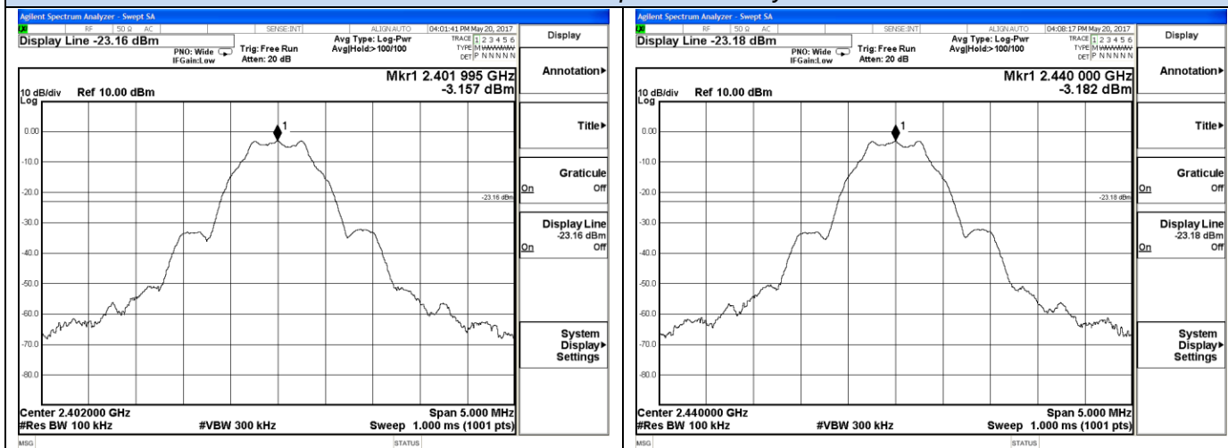
Channel 0 / 2402 MHz
