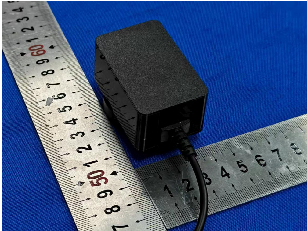
Figure 11. Overall view of Switching Power Supply
