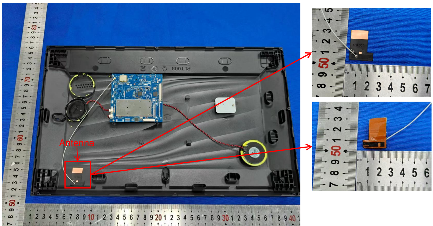
Figure 5. Internal view of unit
