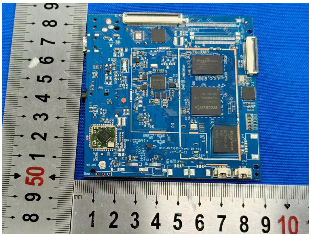
Figure 7. PCB view of unit
