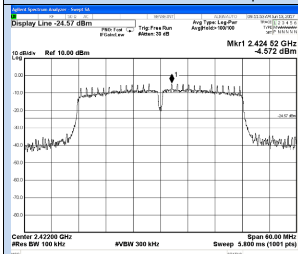
802.11n(HT40)- Low channel Reference
