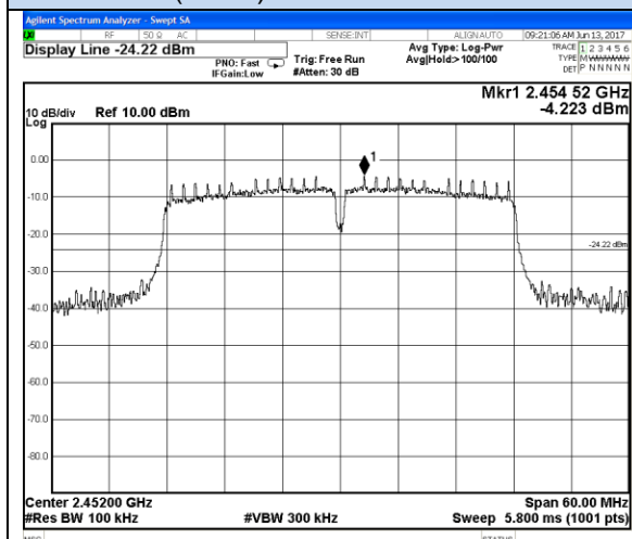
802.11n(HT40)-High channel Reference
