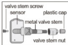
Clamp-In Assembly
