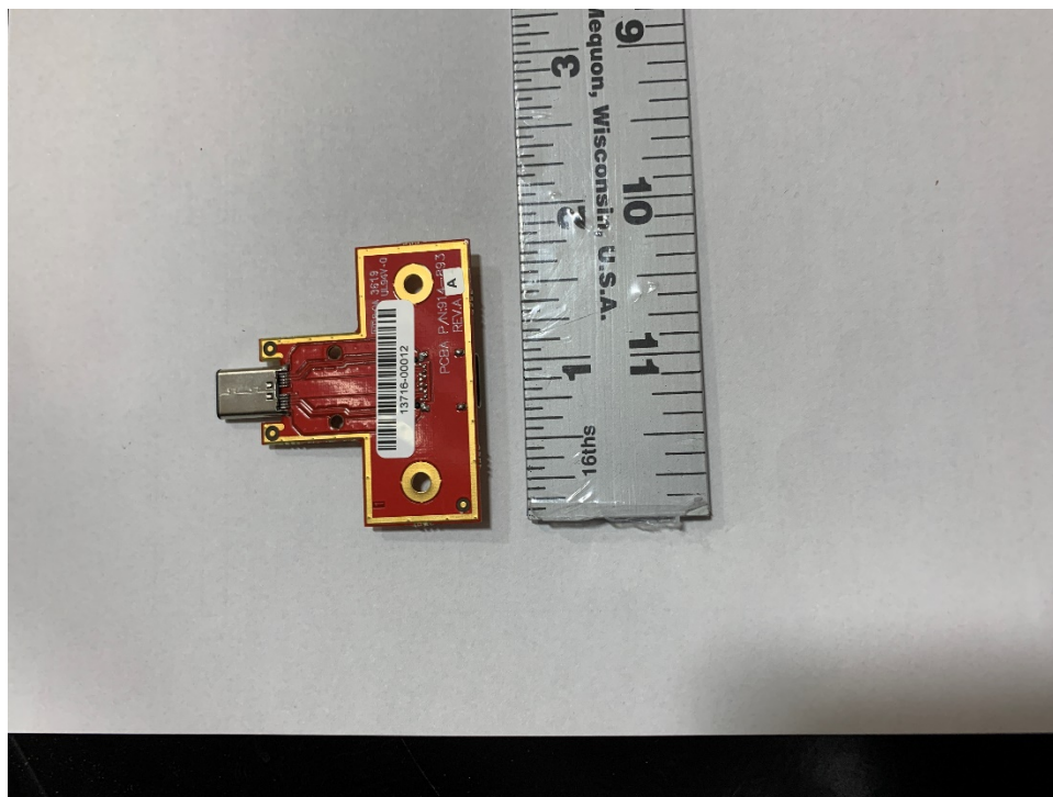
914-893 SSD Board (Front)
