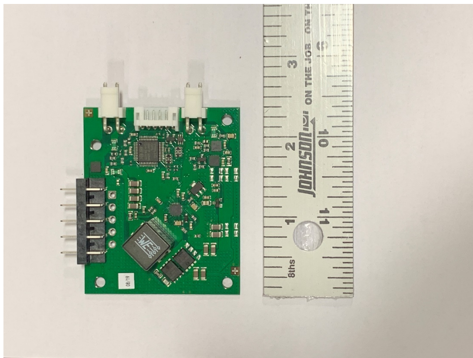
E14-626 Charger Board (Front)
