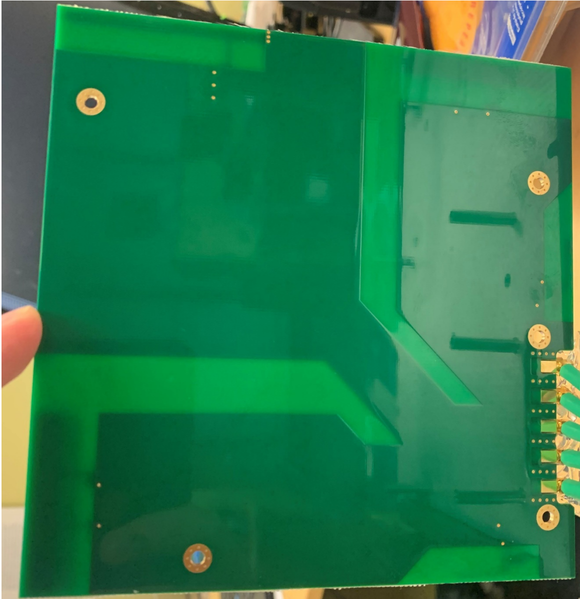
914-907 Antenna Board (bottom)
