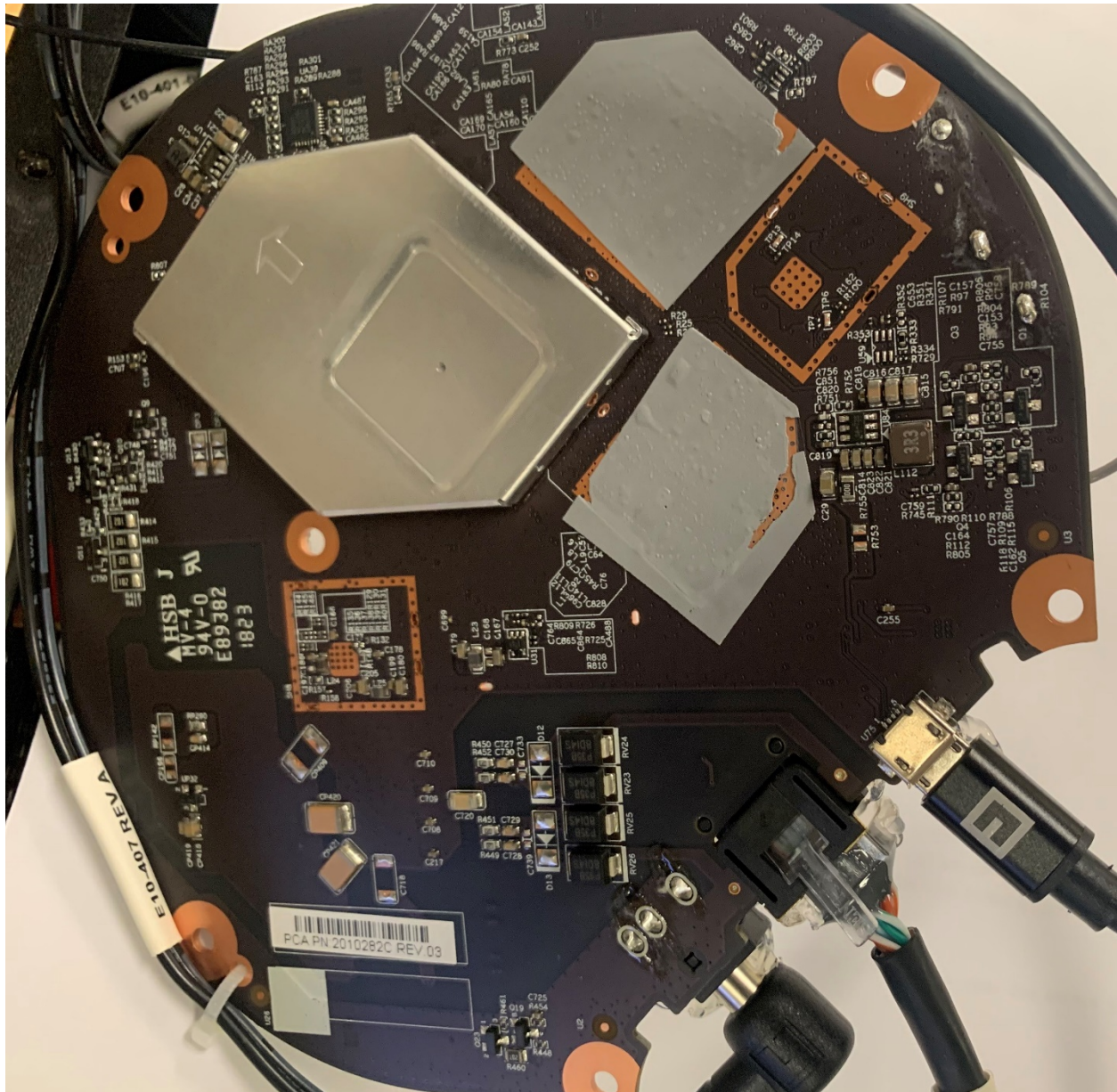
E14-625 Aruba Access Point (bottom)
