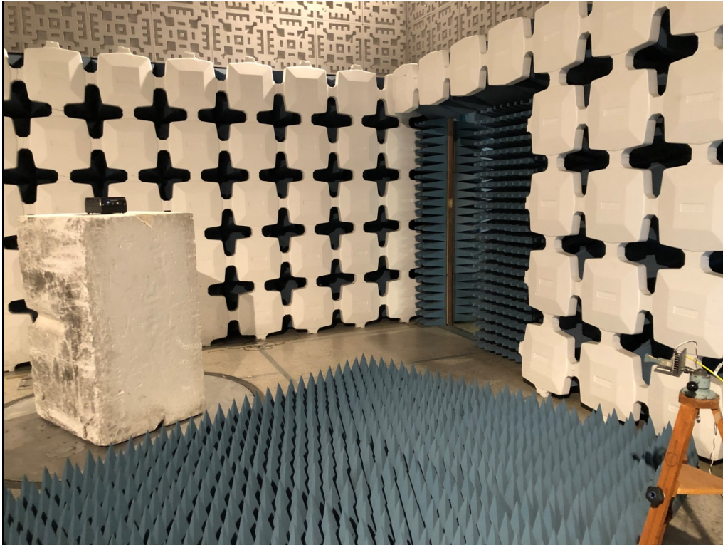
Test Setup for Radiated Spurious Emissions – 18-40GHz Horizontal Antenna Polarization
