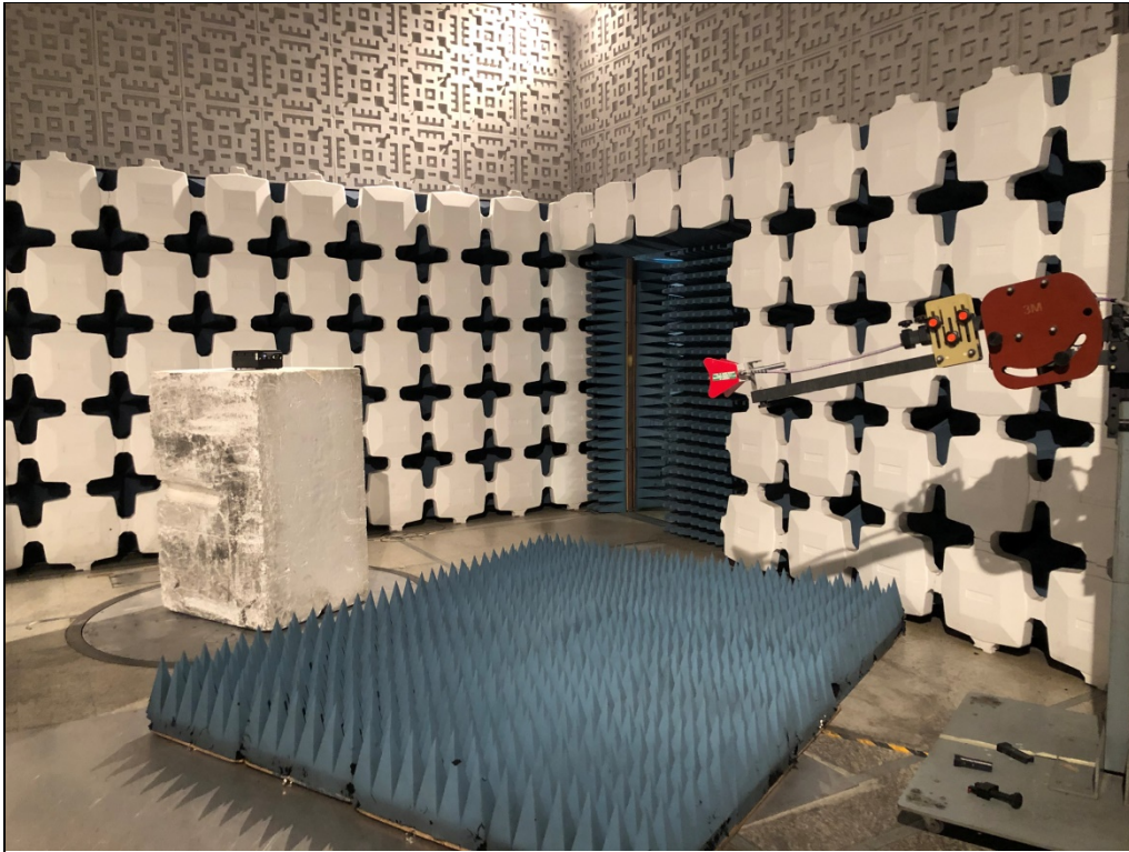
Test Setup for Radiated Spurious Emissions – 1-18GHz Horizontal Antenna Polarization
