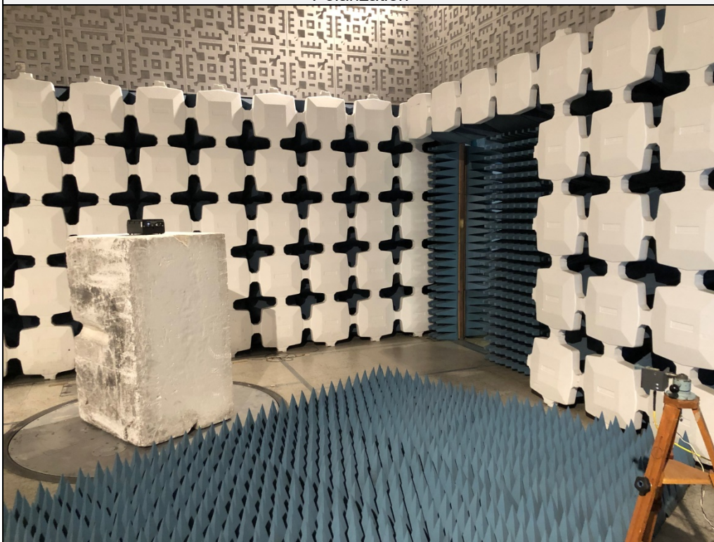
Test Setup for Radiated Spurious Emissions – 18-26.5GHz Vertical Antenna Polarization
