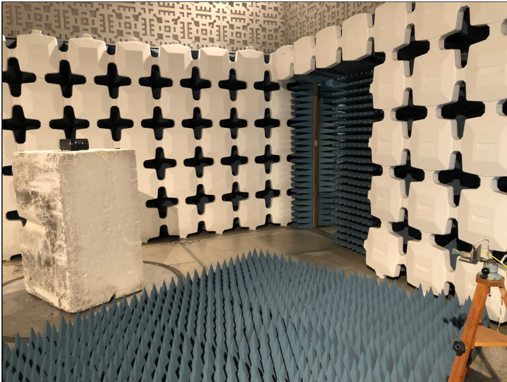
Test Setup for Radiated Spurious Emissions – 18-26.5GHz Horizontal Antenna Polarization
