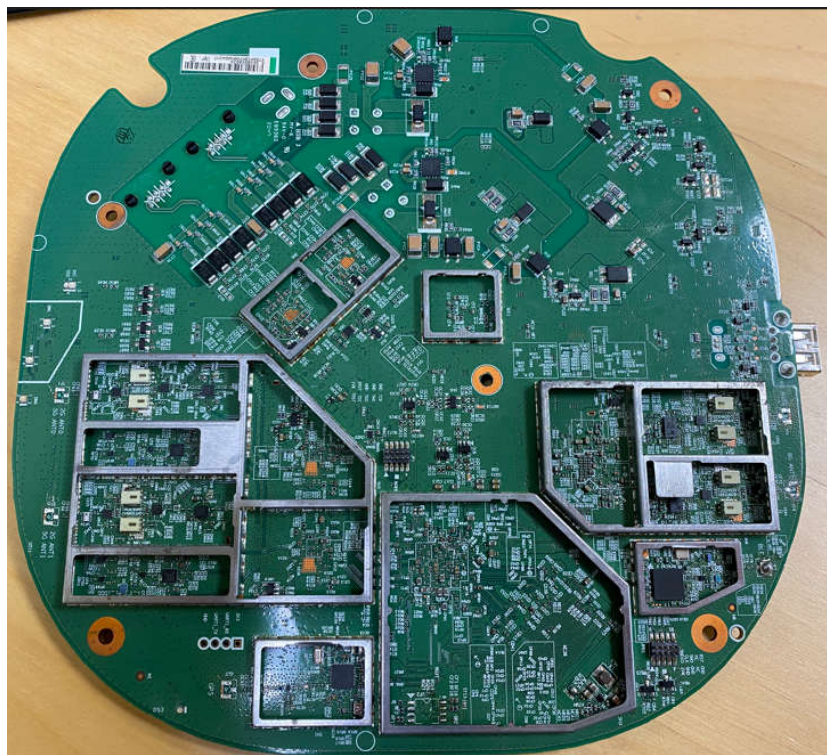
253-00004-000 AP-635 Access Point (bottom) [with shield cans removed]
