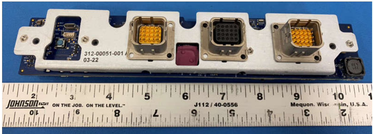
730-00061-001 Serial Interface Board (front)
