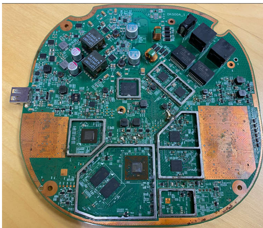
253-00004-000 AP-635 Access Point (top) [with shield cans removed]
