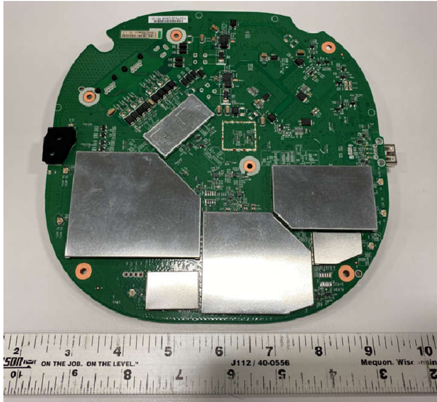
253-00004-000 AP-635 Aruba Access Point (bottom)
