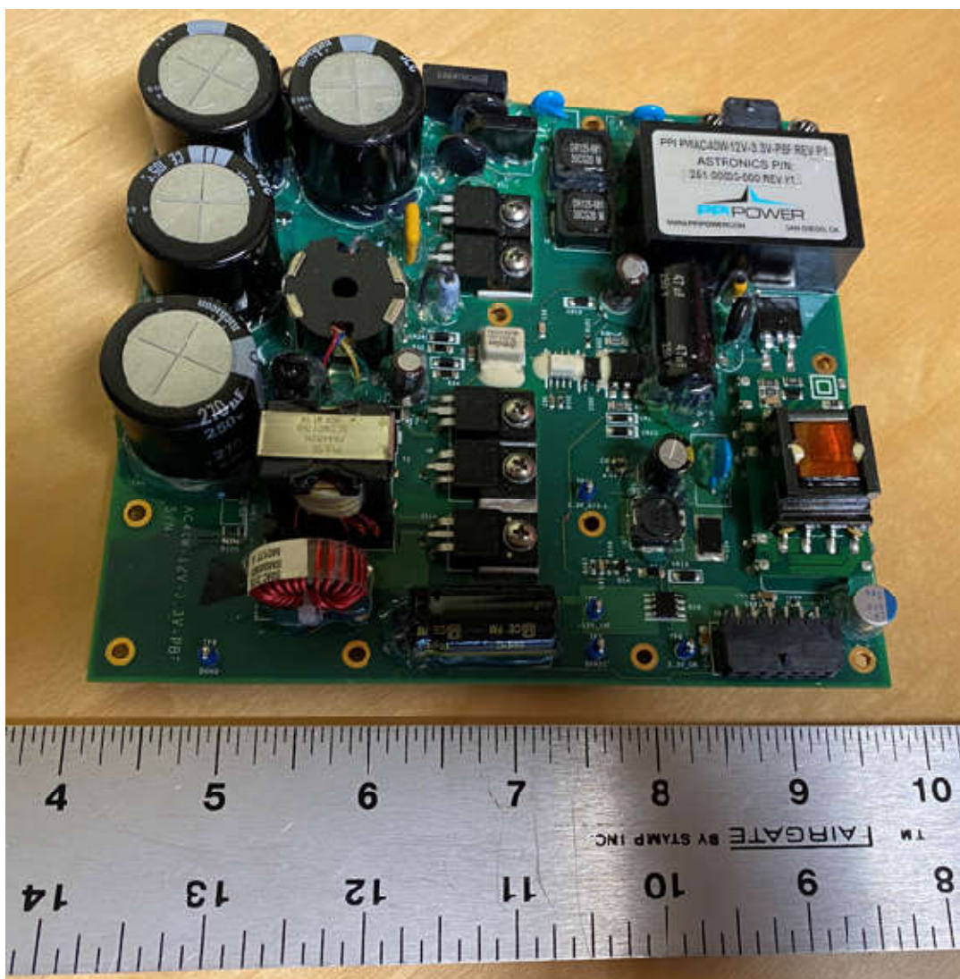
251-00006-000 Power Supply Unit (top)
