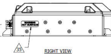
RIGHT VIEW
