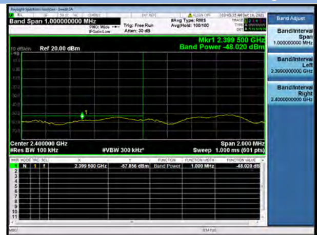
802.11n-20 MHz LOW CHANNEL, Band Edge
