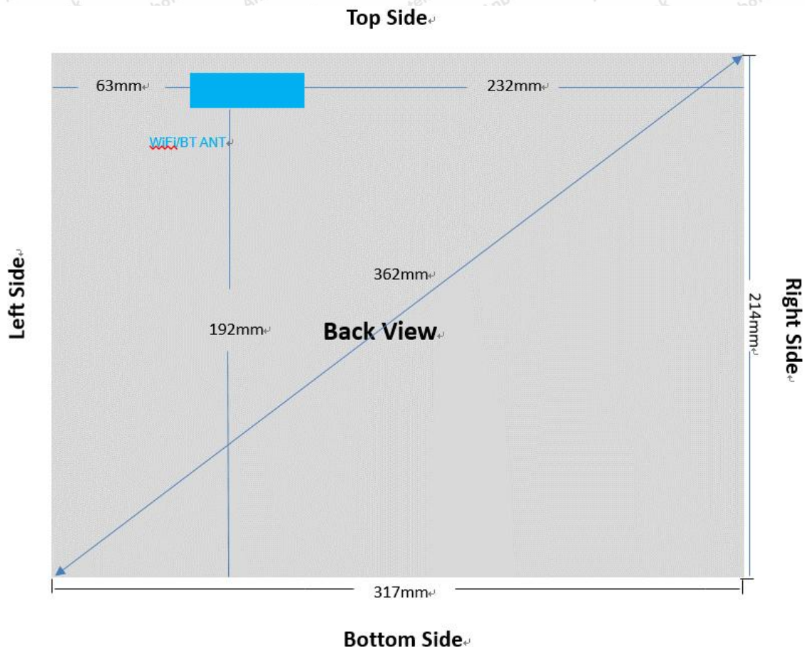
Distance of The Antenna to the EUT surface and edge
