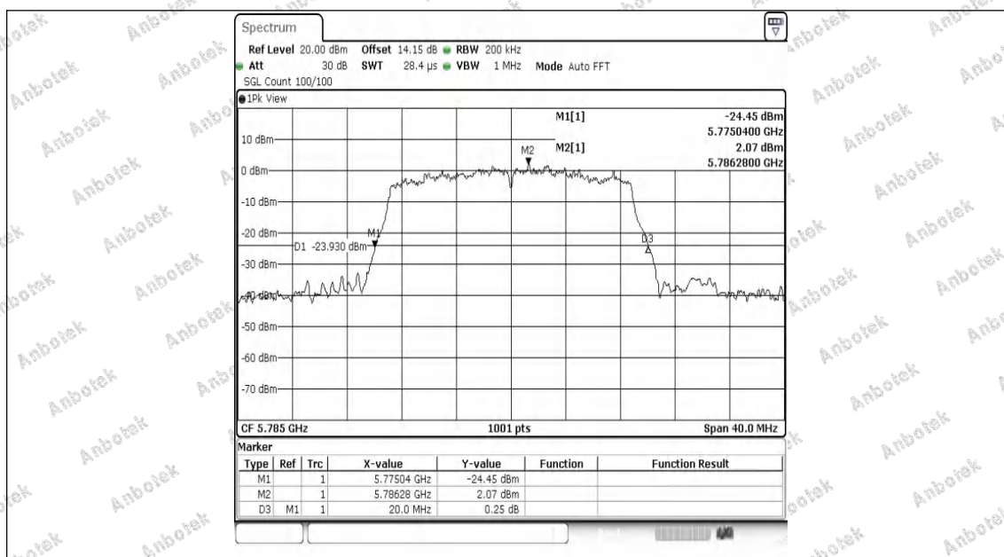
11AC20SISO-Ant1-5785
