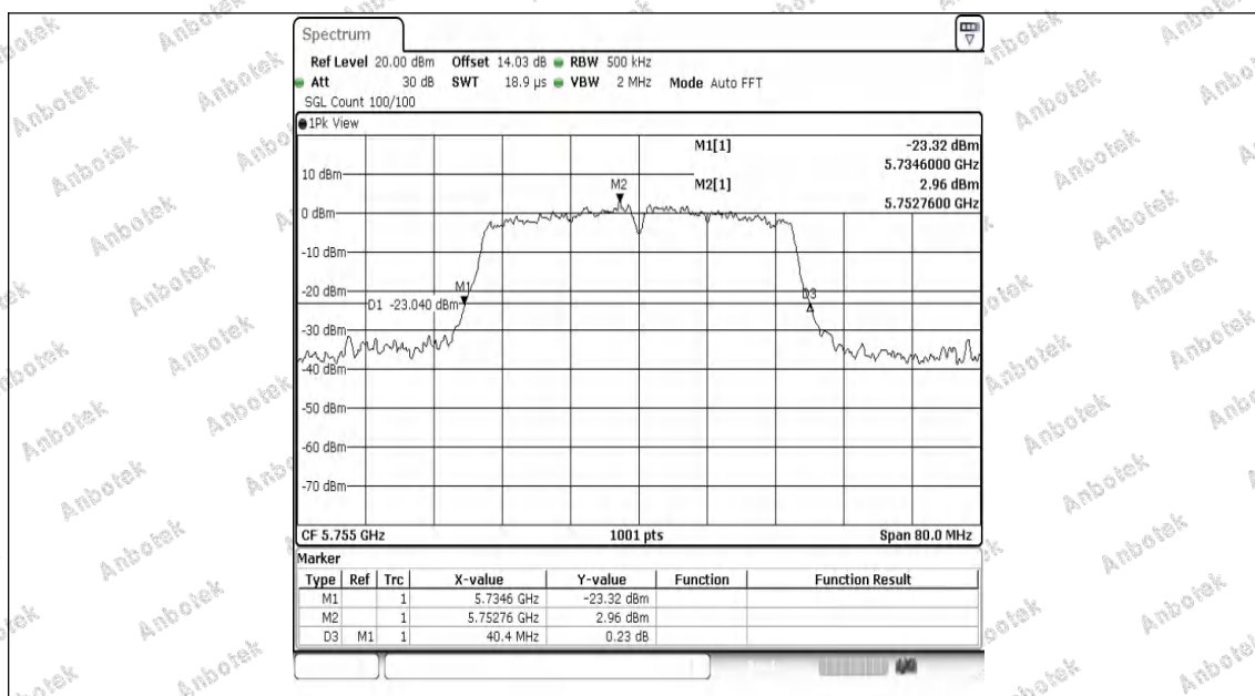
11N40SISO-Ant1-5755
