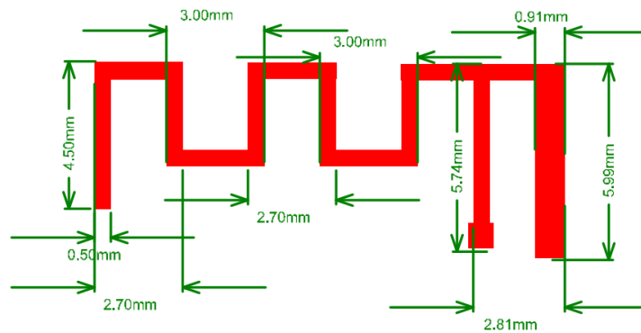
PCB antenna
