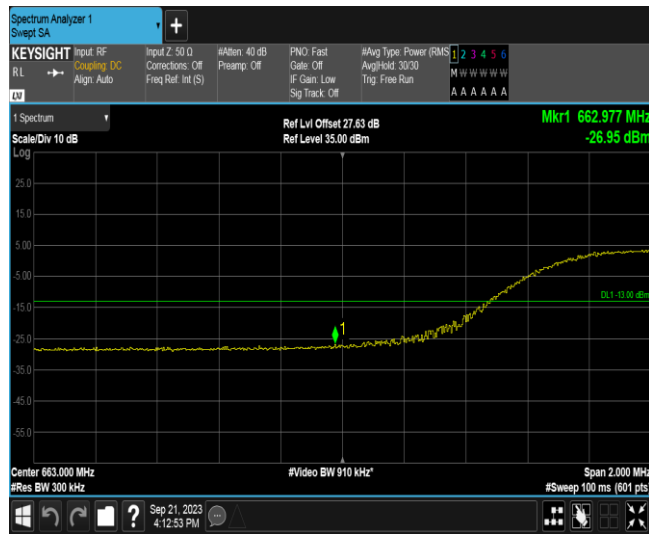
Band71-15MHz-QPSK-133397-1RB#0
