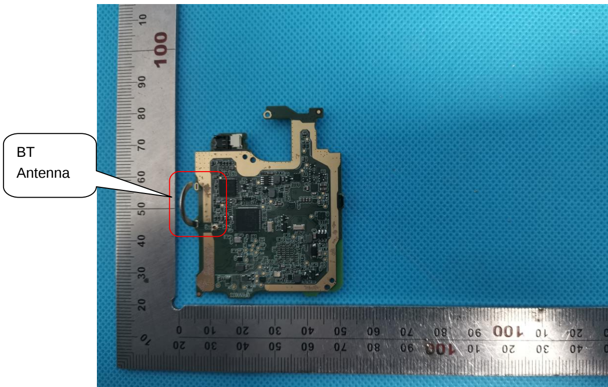
INTERNAL VIEW OF EUT (FIGURE 1)
