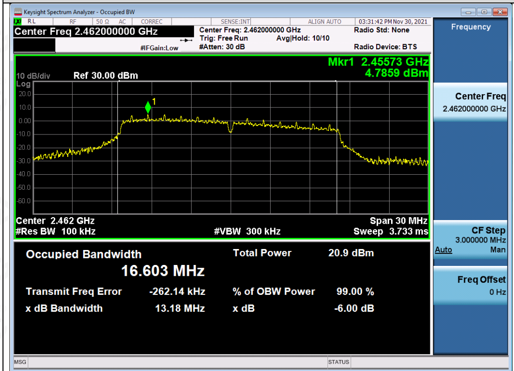
Test_Graph_802.11g_ANT1_2462_6Mbps_DTSBW
