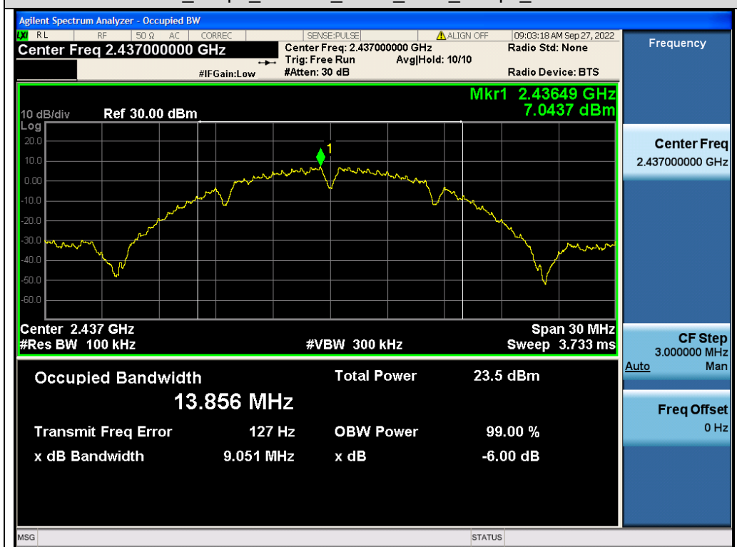
Test_Graph_802.11b_ANT1_2437_1Mbps_DTSBW
