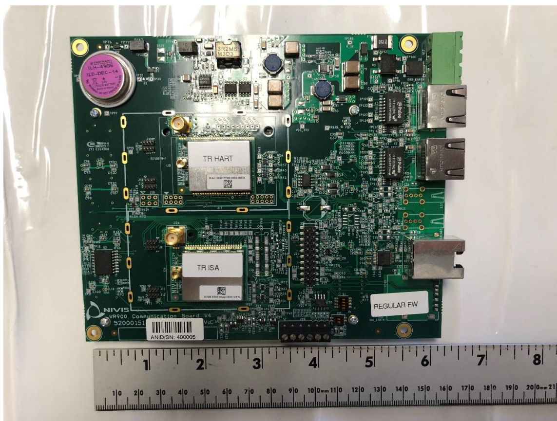
Figure 1. Co-Located Modules on PCB Test Board (VR950)
