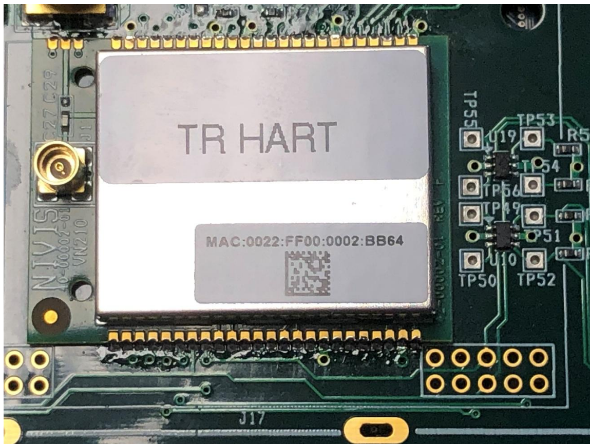
Figure 2. Module Radio 1 for Co-Location
