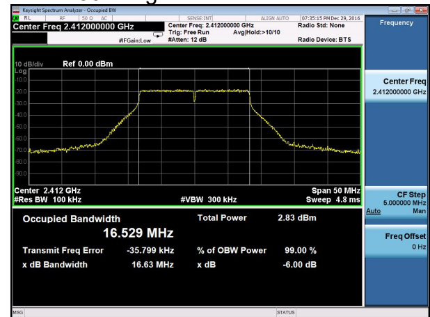
802.11g 2412MHz
